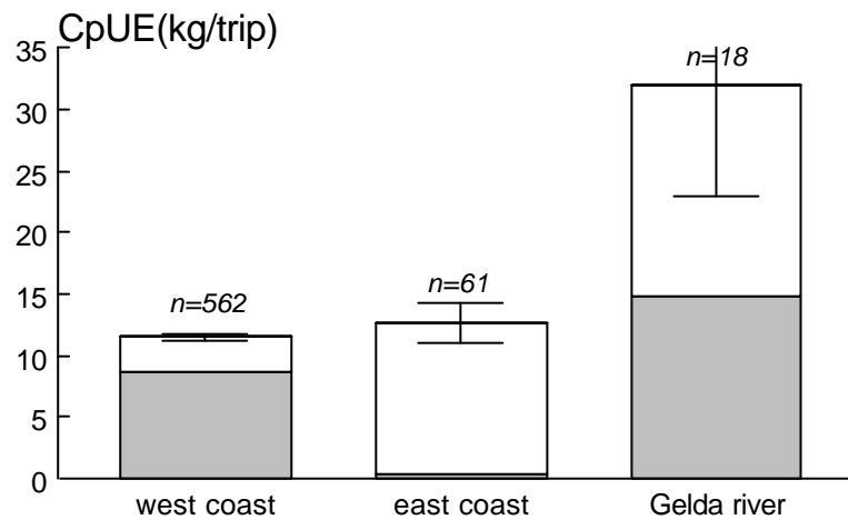
Figure 7.8 Spatial variation of average CpUE (kg-trip -1 ) of reed boat catches per area. Filled bars, O. niloticus , open B. tsanensis
