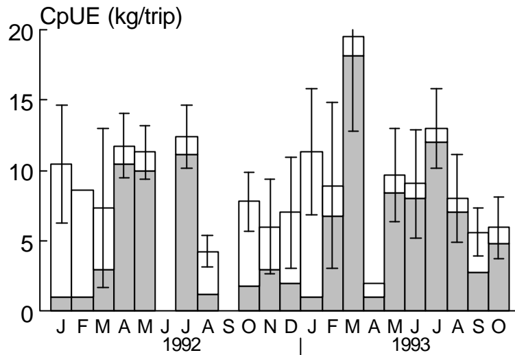
Figure 7.7 Temporal variation (monthly average) of CpUE (kg-trip -1 ) of reed boat catches for southern Lake Tana. Filled bars, O. niloticus , open B. tsanensis
