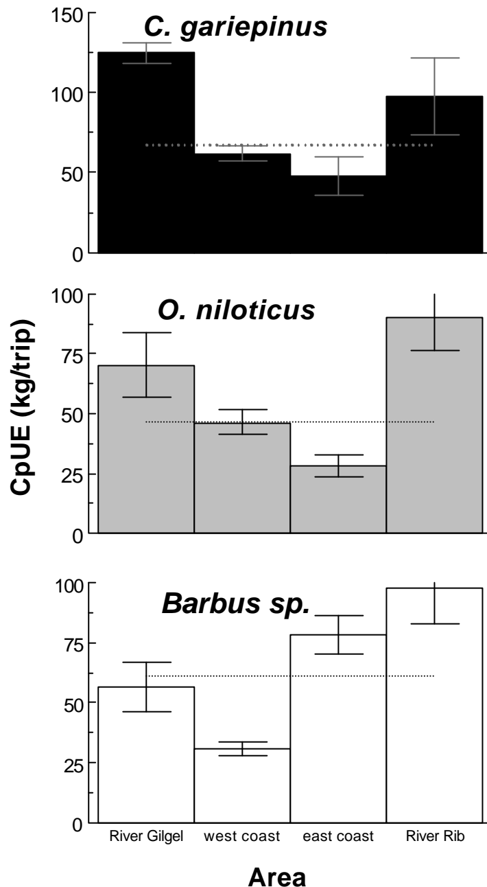
Figure 7.4 Variation of average CpUE ( \text{kg}\cdot\text{trip}^{-1} ) in the various areas for the three major categories in the motorised fishery. The overall means are indicated by the dotted line. Error bars indicate the 95% confidence intervals
