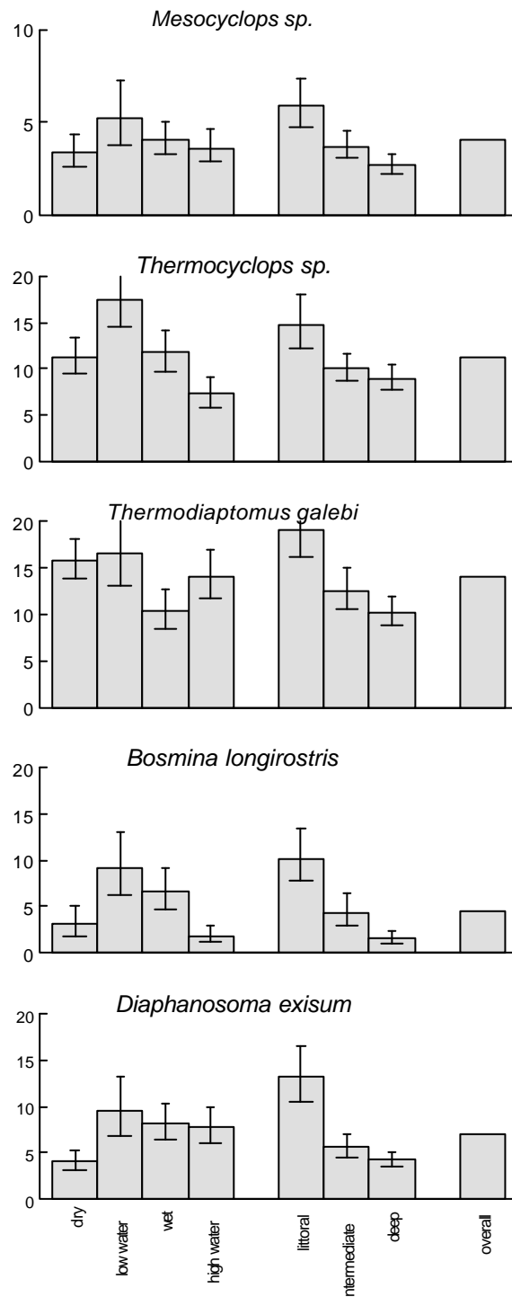
Figure 8.1 Geometric mean densities (N.l -1 ) ( \pm 95% cl) of major zooplankton species per season and area in Bahir Dar Gulf
