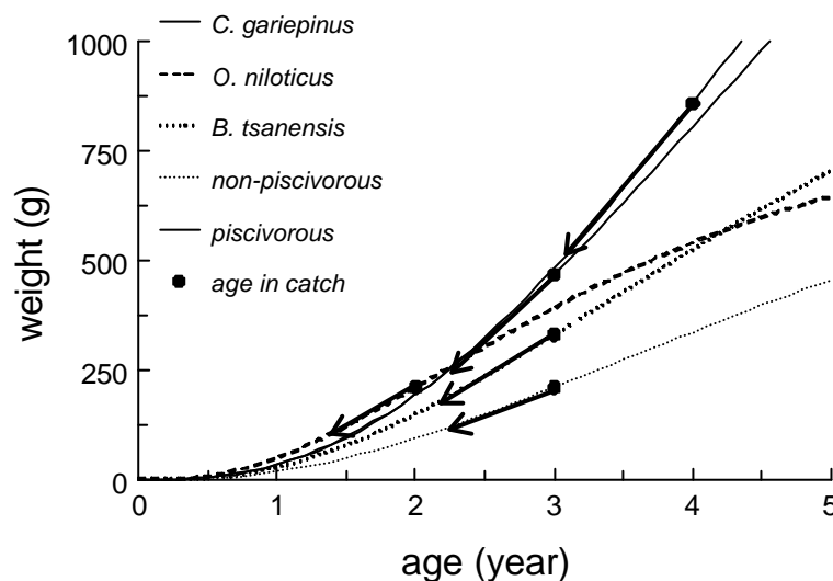
Figure 9.5 Growth curves of the species and groups in the model. Arrows indicate the reduction of their age in the catch when effort would be increased by a factor 5.
