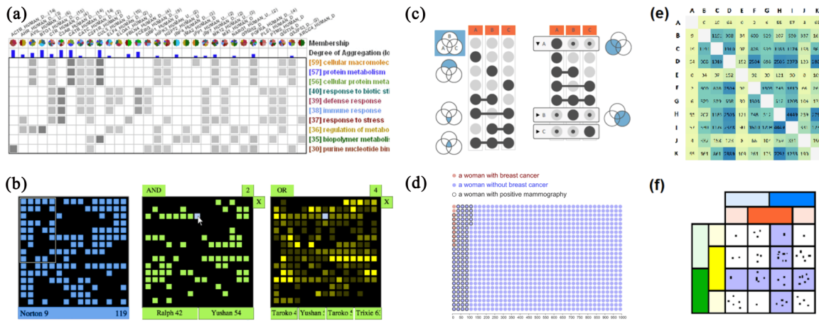
Figure 14: Matrix-based techniques: (a) ConSet [KLS07], (b) OnSet [SMDS14], (c) UpSet [LGS*14], (d) frequency grid [MDF12], (e) similarity matrix [AAMH13], (f) the KMQVL layout [Huo08].
