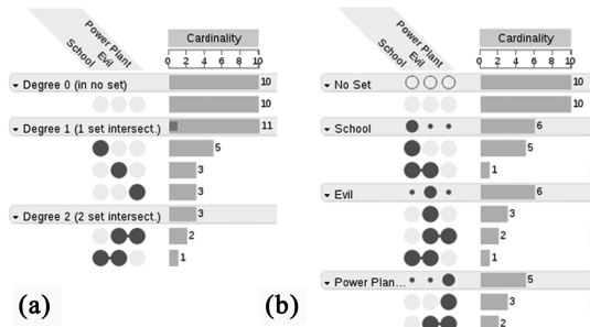
Figure 17: Example grouping options in UpSet [LGS*14]: (a) grouping by element degree, (b) grouping by sets.
