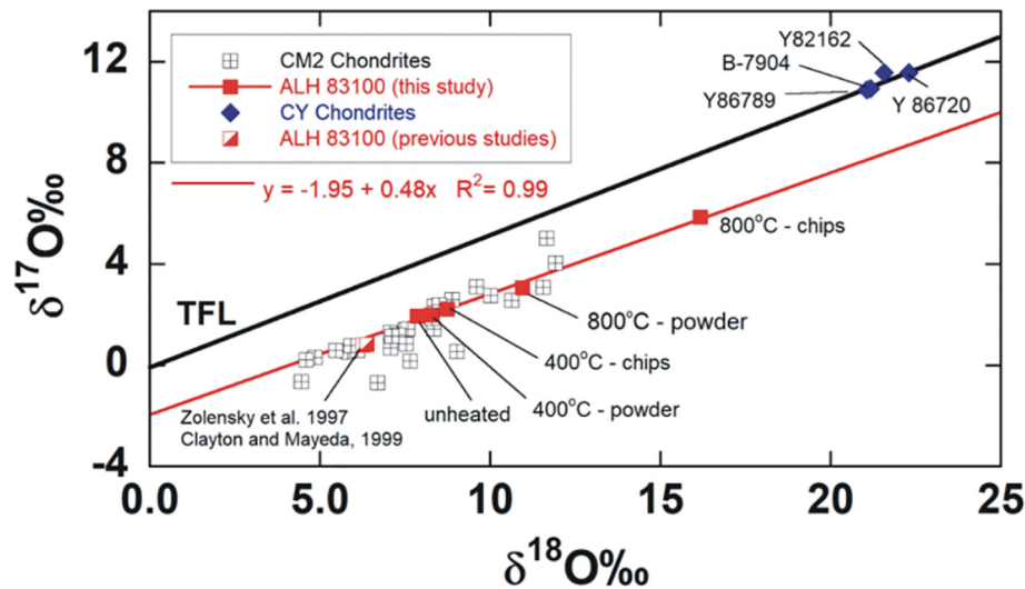
Fig. 4. Oxygen isotopic composition of unheated and heated samples of ALH 83100 compared to previous analyses of ALH 83100 (Zolensky et al., 1997; Clayton and Mayeda, 1999) and other CM2 and CY carbonaceous chondrites (Clayton and Mayeda, 1999; King et al., 2019). A clear implication of this study is that CM2 chondrites cannot be converted into CY chondrites by heating and subsequent dehydration (see text for further discussion).
