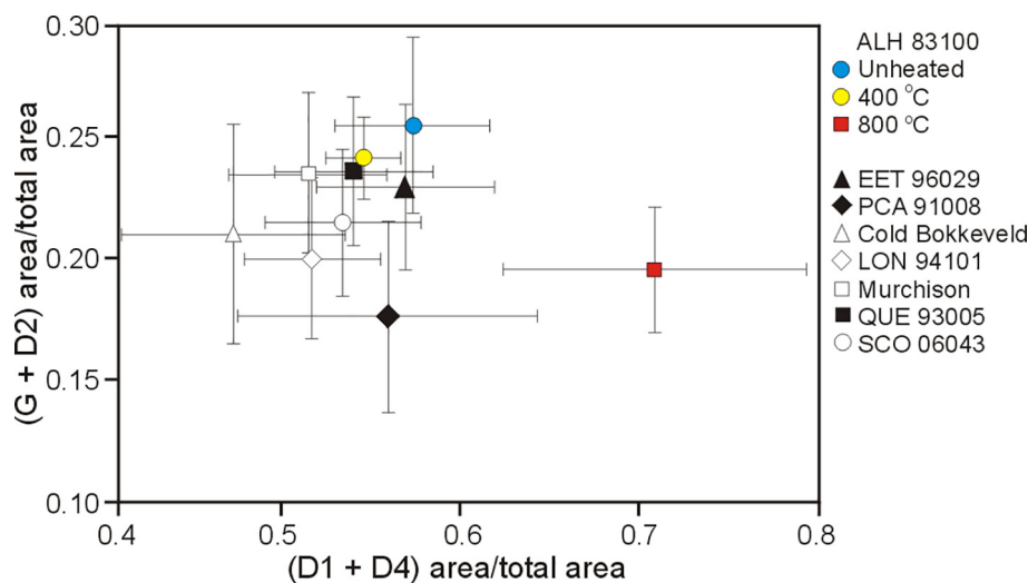
Fig. 12. Results from Raman analyses of carbon in ALH 83100. Shown is the area of the (G + D2) peaks as a proportion of total area (G, D1–4), plotted against the proportional area of (D1 + D4) peaks. Error bars are 1\sigma standard deviation. Plotted along with unheated and heated ALH 83100 are other CMs, both unheated (open symbols) and naturally heated (closed symbols; from Lee et al., 2016). Abbreviations of meteorite names are: EET (Elephant Moraine), PCA (Pecora Escarpment), LON (Lonewolf Nunataks), QUE (Queen Elizabeth Range), SCO (Scott Glacier). The number of spectra analysed from each sample are: ALH 83100 unheated ( n = 27 ), 400 °C ( n = 38 ), 800 °C ( n = 34 ), EET 96029 ( n = 49 ), PCA 91008 ( n = 22 ), Cold Bokkeveld ( n = 45 ), LON 94101 ( n = 40 ), Murchison ( n = 43 ), QUE 93005 ( n = 43 ), SCO 06043 ( n = 40 ).
