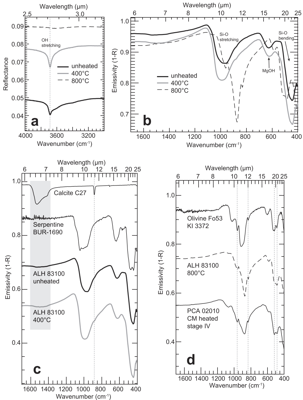
Fig. 3. (a and b) IR spectra of unheated and heated chips in thin section. Spectra are not offset or scaled. Vertical dotted line in (a) marks the OH band emission maximum (reflectance minimum) at 3684\text{ cm}^{-1} ( 2.71\text{ }\mu\text{m} ) (c) The spectral shapes of both the unheated and 400^\circ chips are similar to the emission spectrum of FeMg serpentine, with weak spectral features consistent with calcite. (d) The 800^\circ chip shows spectral features consistent with Fe-bearing olivine, and is also similar to the spectrum of naturally heated (stage IV) CM PCA 02010 (from Hanna et al., 2020 ). Spectra in (c) and (d) scaled and offset for clarity and vertical dotted lines indicate spectral features due to calcite (c) and Fe-bearing olivine (d).
