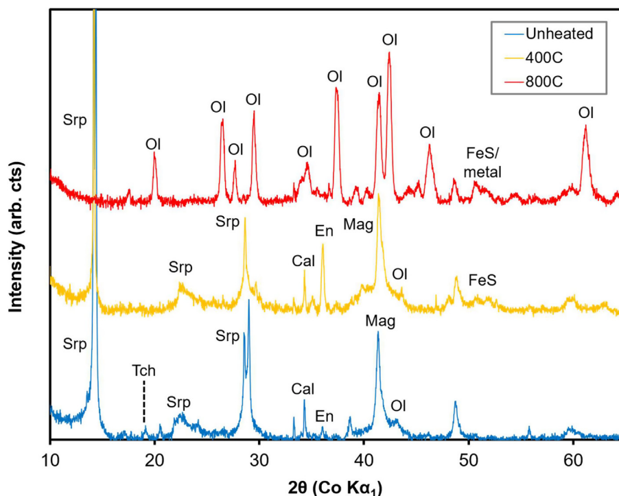
Fig. 2. XRD patterns of unheated and heated ALH 83100 collected using a PANalytical X'Pert Pro scanning XRD. Only patterns from the samples that were heated as chips then powdered are shown. Srp = serpentine; Mag = magnetite; Cal = calcite; Ol = olivine; En = enstatite; Tch = tochilinite.
