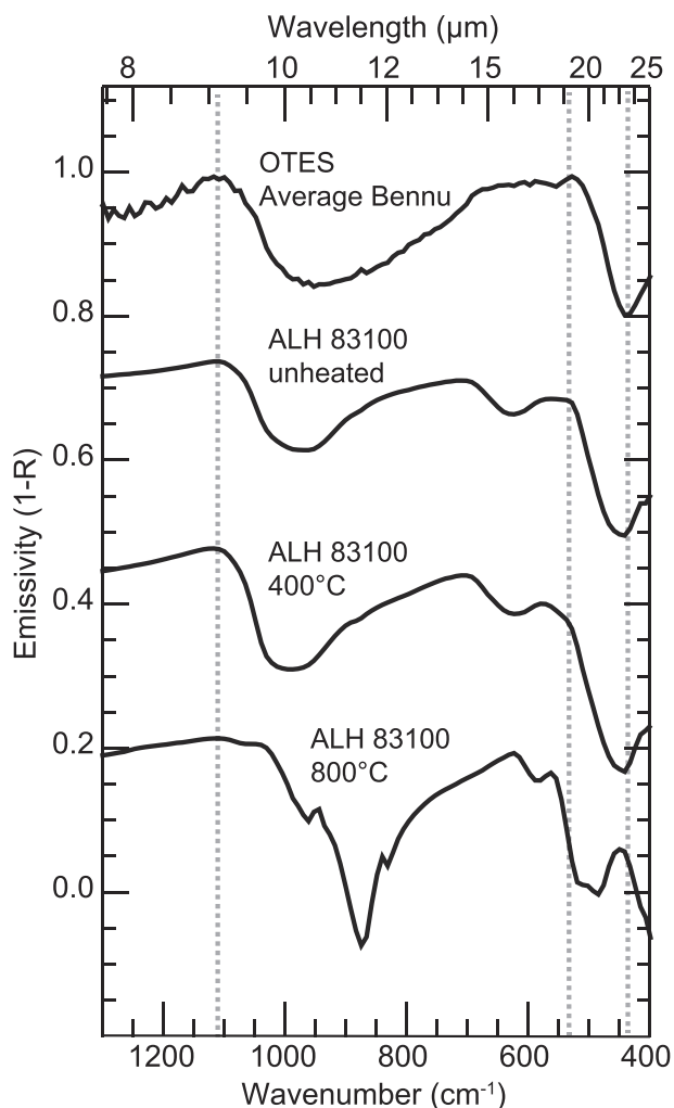
Fig. 13. Global average Benu OTES spectrum from Hamilton et al. (2019) plotted with spectra from the present study. Spectra have been offset for clarity, and the Benu spectrum has been scaled for comparison to the laboratory spectra. Dotted lines highlight that the CF, emissivity maximum near 530\text{ cm}^{-1} ( 18.9\text{ }\mu\text{m} ), and Si–O bending minimum of the Benu spectrum more closely match unheated or mildly heated ALH 83100, although the wider Si–O stretching band and weaker Mg–OH band of the 400\text{ }^{\circ}\text{C} sample are more consistent with Benu's spectral shape.
