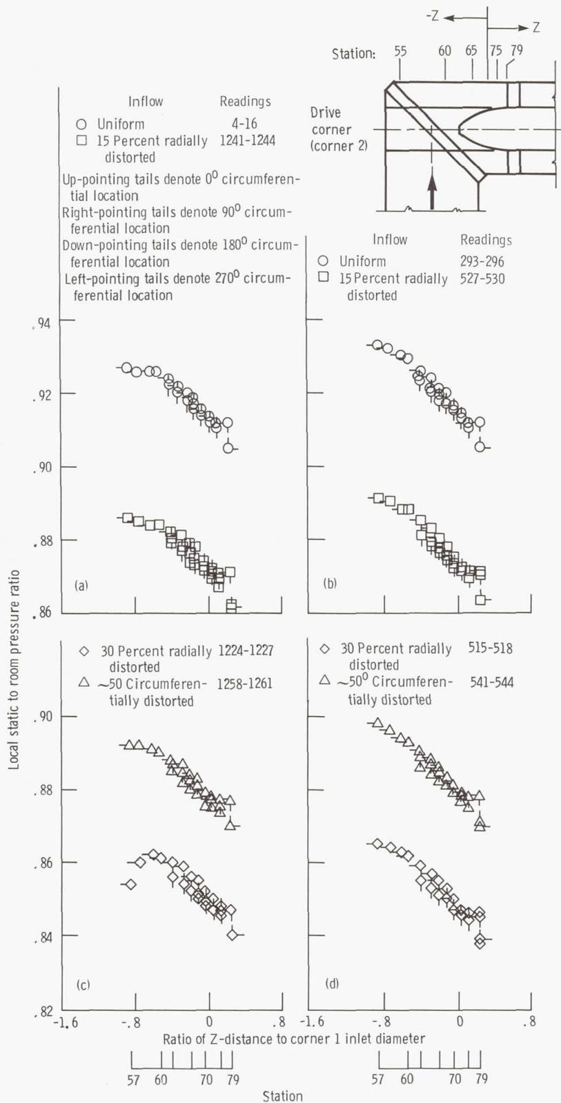
(a) Vanes A4 in corner 2, comparing uniform and 15-percent radially distorted inflow. (b) Vanes B in corner 2, comparing uniform and 15-percent radially distorted inflow. (c) Vanes A4 in corner 2, comparing 30-percent radially distorted and ~50° circumferentially distorted inflow. (d) Vanes B in corner 2, comparing 30-percent radially distorted and ~50° circumferentially distorted inflow.
