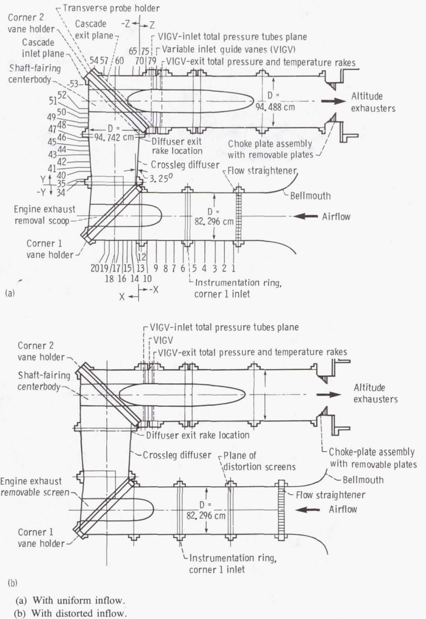
Figure 3.—Schematic of corner 1-corner 2 test apparatus.
