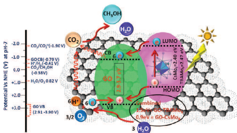
Fig. 9 Plausible mechanism of photoreduction of \text{CO}_2 into methanol catalyzed by GO-hexamolybdenum composite
