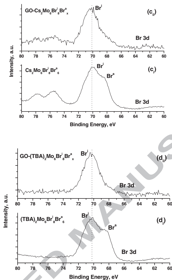
Fig 4: XPS spectra of (a) Cs 3d; (b) Mo 3d; (c) Br 3d regions for \text{Cs}_2\text{Mo}_6\text{Br}_8\text{Br}_x^{\text{a}} and \text{GO-Cs}_2\text{Mo}_6\text{Br}_8\text{Br}_x^{\text{a}} ; (d) Br 3d regions for (\text{TBA})_2\text{Mo}_6\text{Br}_8\text{Br}_x^{\text{a}} and \text{GO-(TBA)}_2\text{Mo}_6\text{Br}_8\text{Br}_x^{\text{a}} composites.
