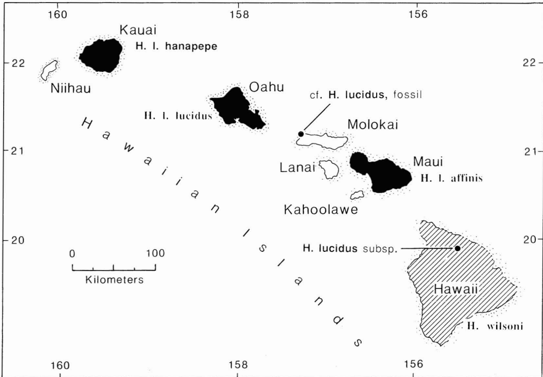
FIGURE 1. Generalized known distribution of Hemignathus wilsoni (hatched) and the forms of H. lucidus (black), including probable fossil record from Moloka'i and that from the island of Hawai'i reported here.
