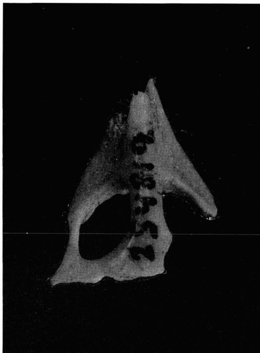
Figure 3. Dorsal view of a fossil rostrum (USNM 254819) referred to Hemignathus lucidus , from sand dune deposits at 'Īlio Point, Moloka'i. The specimen lacks most of the premaxillary symphysis and part of the margin of the right nostril.
