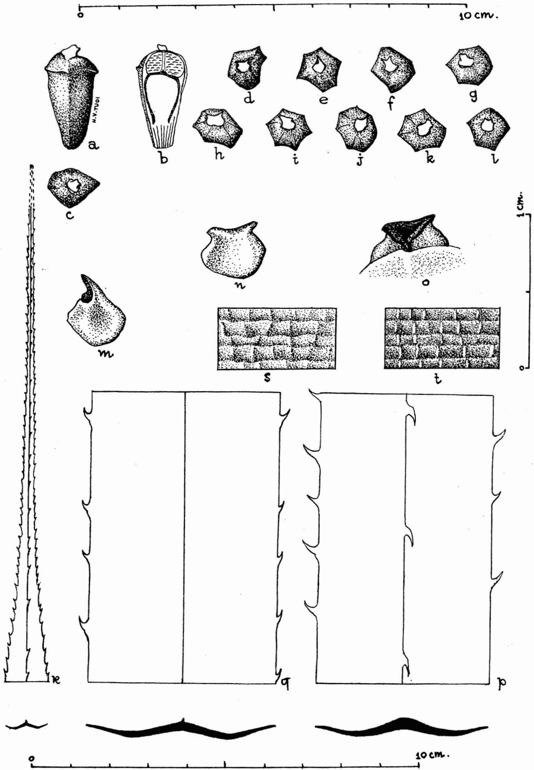
FIG. 201. Pandanus reticulosus St. John, from holotype. a , Drupe, lateral view, \times 1 ; b , drupe, longitudinal median section, \times 1 ; c-l , drupe, apical view, \times 1 ; ( d and f are the most common kinds; e is basal, rarely lateral); m , apex of apical drupe and stigma, lateral view, \times 4 ; n , apex of lateral drupe, oblique view, \times 4 ; o , apex of lateral drupe and stigma, proximal view, \times 4 ; p , leaf base, lower side, \times 1 ; q , leaf middle, lower side, \times 1 ; r , leaf apex, lower side, \times 1 ; s , leaf middle, upper side, secondary and tertiary veins, \times 4 ; t , leaf middle, lower side, secondary and tertiary veins, \times 4 .
