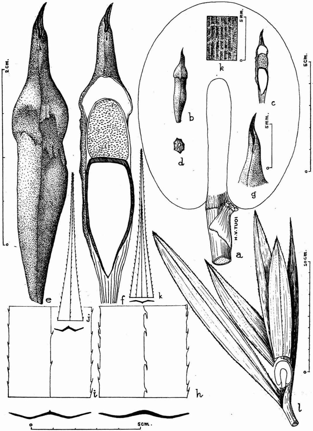
FIG. 192. Pandanus biplicatus St. John, from holotype. a , Syncarp profile, \times 1 ; b , drupe, lateral view, \times 1 ; c , drupe, longitudinal median section, \times 1 ; d , drupe, apical view, \times 1 ; e , drupe, lateral view, \times 4 ; f , drupe, longitudinal median section, \times 4 ; g , style and stigma, distal view, \times 4 ; h , leaf base, lower side, \times 1 ; i , leaf middle, lower side, \times 1 ; j , leaf apex, lower side, \times 1 ; k , leaf apex, upper side, \times 1 ; l , young pistillate inflorescence, lateral view, \times \frac{1}{2} .
