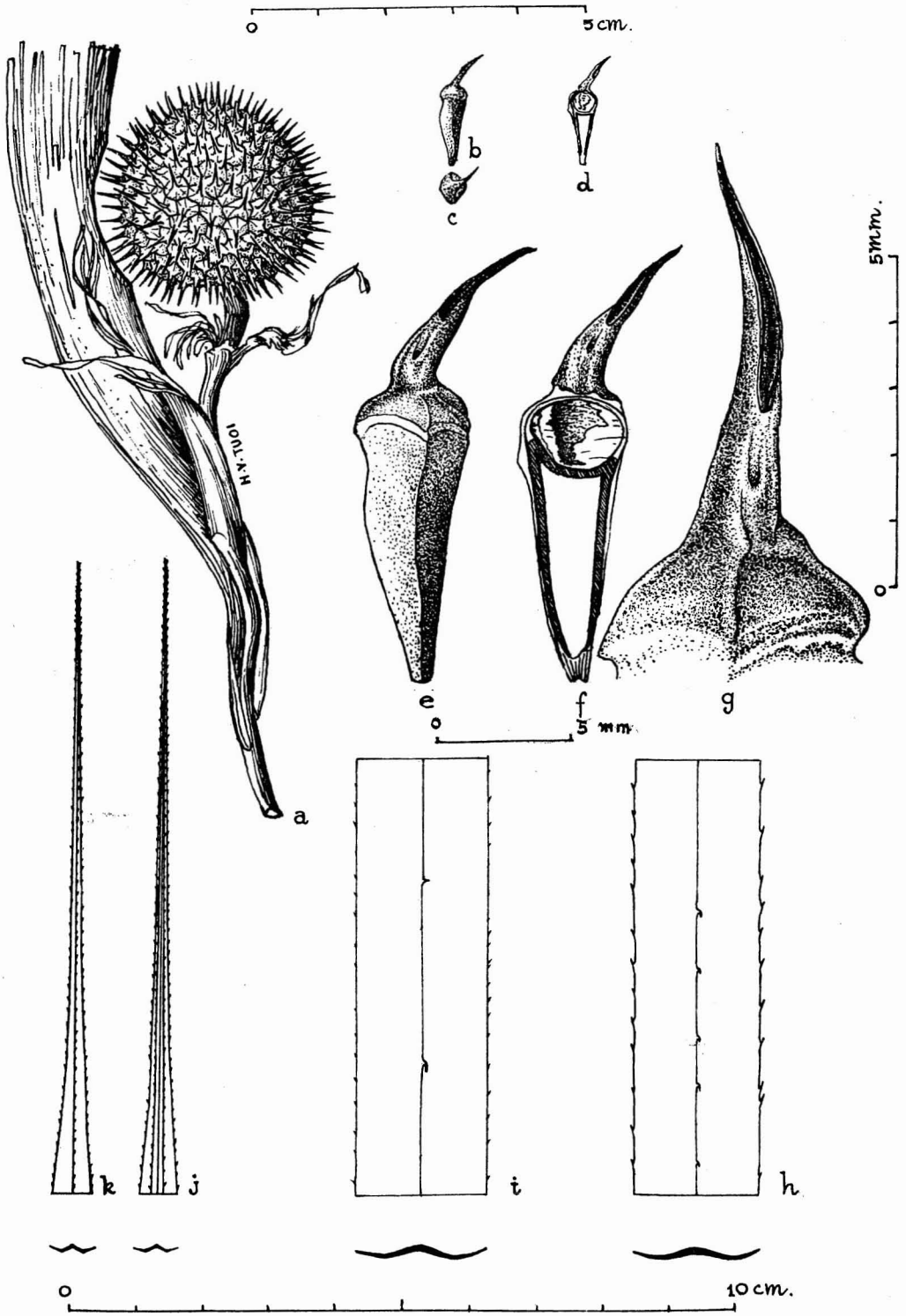
FIG. 193. Pandanus Toei St. John, from holotype. a , Peduncle and syncarp, \times 1 ; b , drupe, lateral view, \times 1 ; c , drupe, apical view, \times 1 ; d , drupe, longitudinal median section, \times 1 ; e , drupe, lateral view, \times 4 ; f , drupe, longitudinal median section, \times 4 ; g , style and stigma, distal view, \times 10 ; h , leaf base, lower side, \times 1 ; i , leaf middle, lower side, \times 1 ; j , leaf apex, upper side, \times 1 ; k , leaf apex, lower side, \times 1 .
