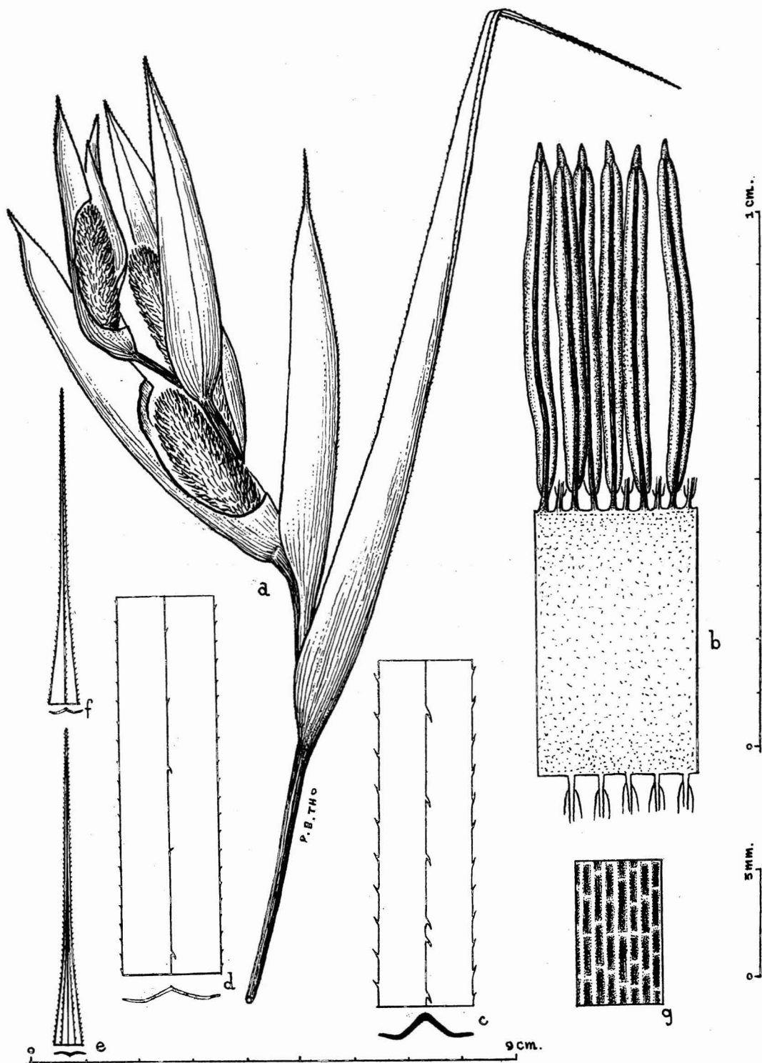
FIG. 194. Pandanus Toei St. John, from Smitinand 1,391. a , Staminate inflorescence, \times 1 ; b , axis and stamens, \times 10 ; c , leaf base, lower side, \times 1 ; d , leaf middle, lower side, \times 1 ; e , leaf apex, upper side, \times 1 ; f , leaf apex, lower side, \times 1 ; g , secondary longitudinal veins and tertiary cross veins, at midsection, lower side, \times 4 .
