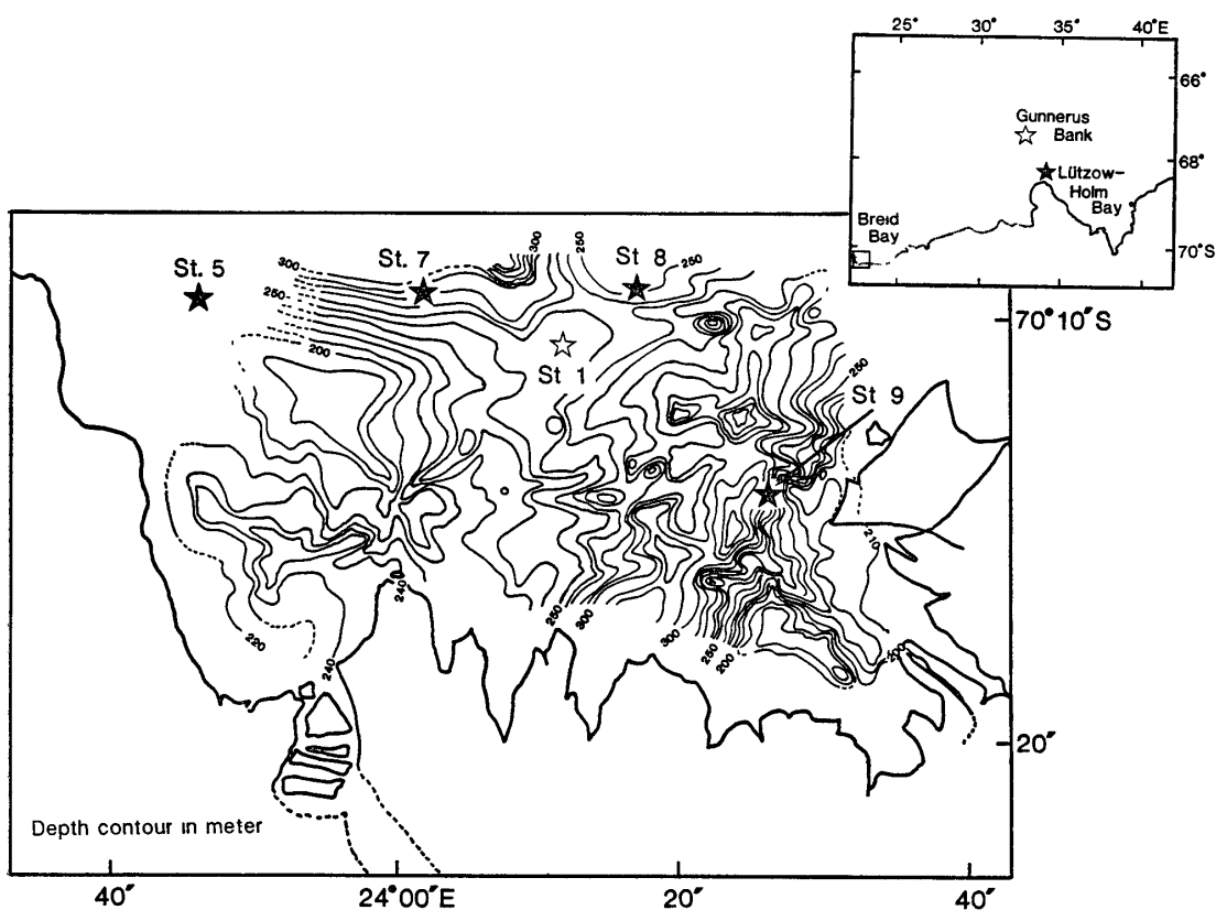
Fig 1 Trawling sites (stars) in Breid Bay and Günnerus Bank by the icebreaker "Shirase" (★, December 1984 to February 1985, ☆, December 1985 to February 1986)
