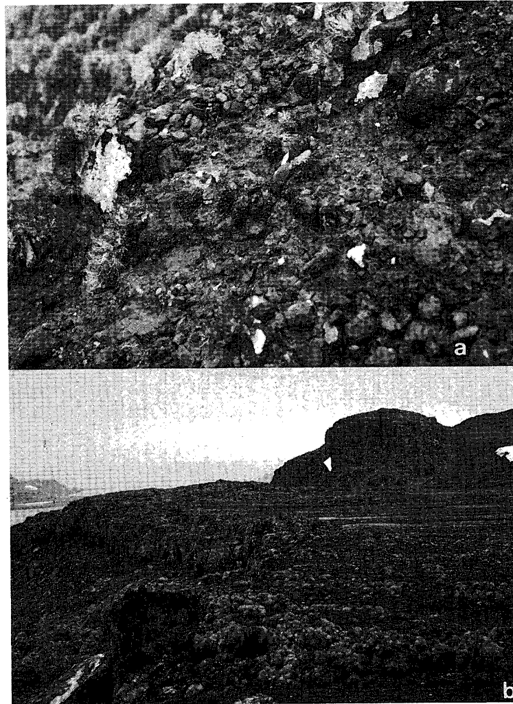
Fig. 5. a : Dermatomycarpon cf. intestiniforme with Usnea aurantiacoatra growing in the well-irrigated rocky slopes. b : Characteristic "irrigated" landscape in the maritime Antarctic, the Fildes Peninsula. ( a : 24. II. 1989; b : 22. II. 1989).
