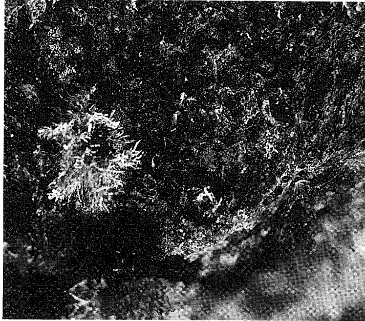
Fig. 4. Umbilicaria decussata (foliose) growing with Himantormia lugubris (fruticose, black) and Usnea aurantiacoatra (fruticose, whitish). (Fildes Peninsula, 16. II. 1989).
