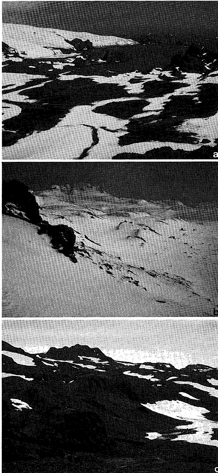
Fig. 3. a : Northwestern part of Harmony Cove; b , c : Southeastern part of the Fildes Peninsula. They have heavy snow in winter, but snow melts rapidly during spring to summer. ( a : 4. I. 1989; b : 14. XI. 1988; c : 21. I. 1989).
