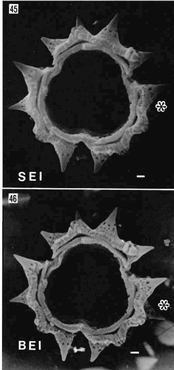
Fig. 45–46. Cryomicrotomy and electron imaging of Espelitia schultzii (Asteraceae). The frozen and sectioned exine was imaged with secondary (SEI) (Fig. 45) and backscatter (BEI) (Fig. 46) detector systems. These comparative micrographs demonstrate the much greater depth of focus obtained with BEI. Note that spine features (opposite asterisks) are nearly unresolved with secondary imaging. General exine details are also considerably enhanced with BEI. (The scales equal 1 \mu\text{m} .)
