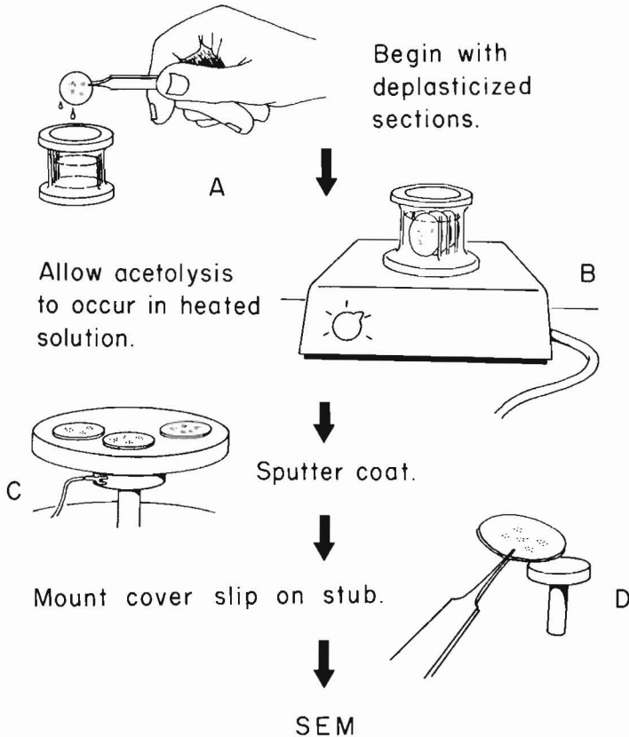
Fig. 100. Coverslip acetolysis method.—A. Start with sections of unacetolyzed pollen with epoxy embedding media removed by deplastitization method.—B. Coverslips with attached pollen sections are placed in a Pyrex coplin jar containing acetolysis solution and carefully heated on a hot plate for 5 min.—C. After removal from acetolysis solution, rinsing and drying, the coverslips are sputter coated.—D. Coverslips are sealed to specimen stub and placed in SEM for examination and photography.
