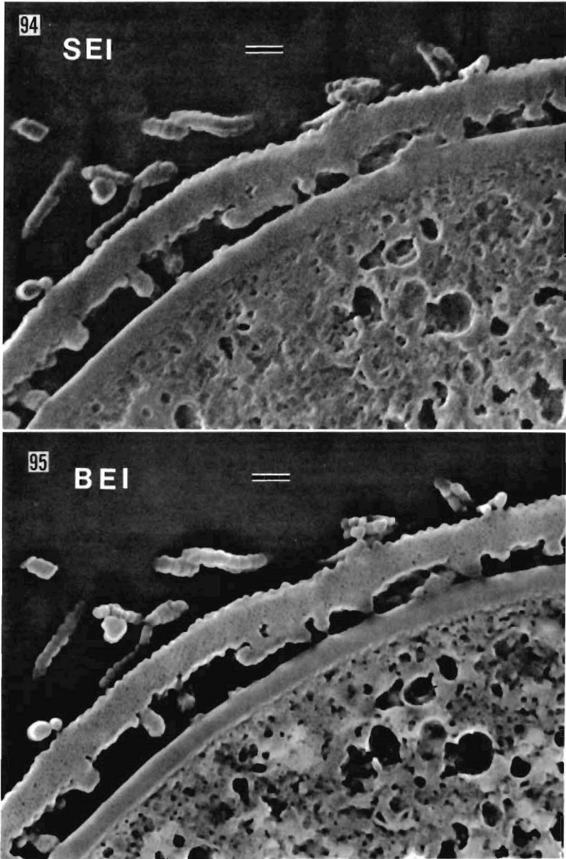
Fig. 94–95. Thick-section deplastization method using Camissonia cardiophylla ssp. robusta (Onagraceae) pollen and illustrated with secondary and backscatter detector systems.—94. Section ( \frac{1}{4} – \frac{1}{2} \mu\text{m} thick) deplastitized and examined with secondary electron detector system (SEI).—95. Identical section examined with backscatter electron detector system (BEI). Comparison of all exine components (viscin threads, exine, cytoplasm) by both detectors dramatically indicates the superior detail obtained with backscatter electron imaging. (The scales equal 1 \mu\text{m} .)
