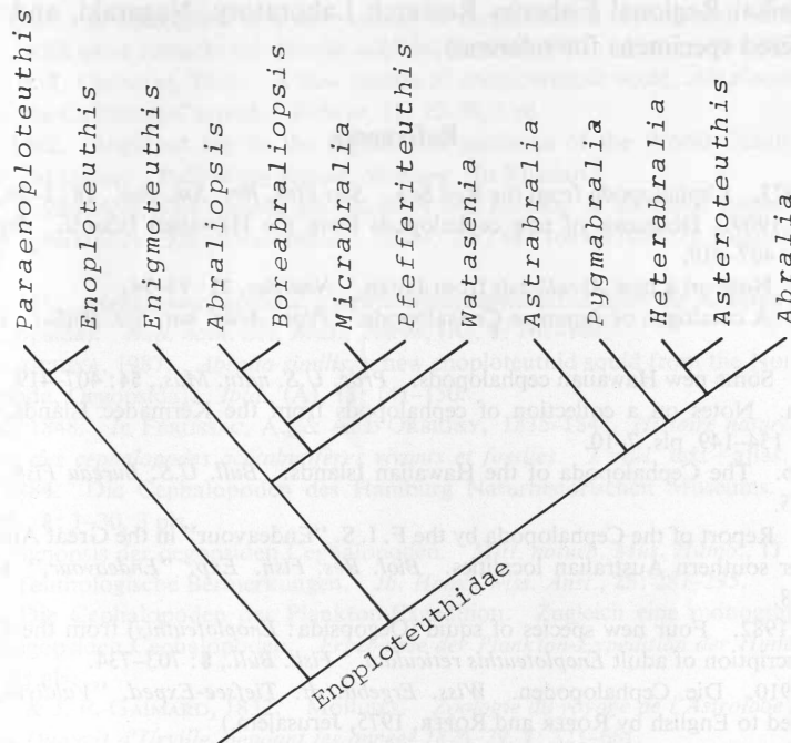
Fig. 29. Possible phylogenetic relationships of genera and subgenera of the Family Enoploteuthidae.
