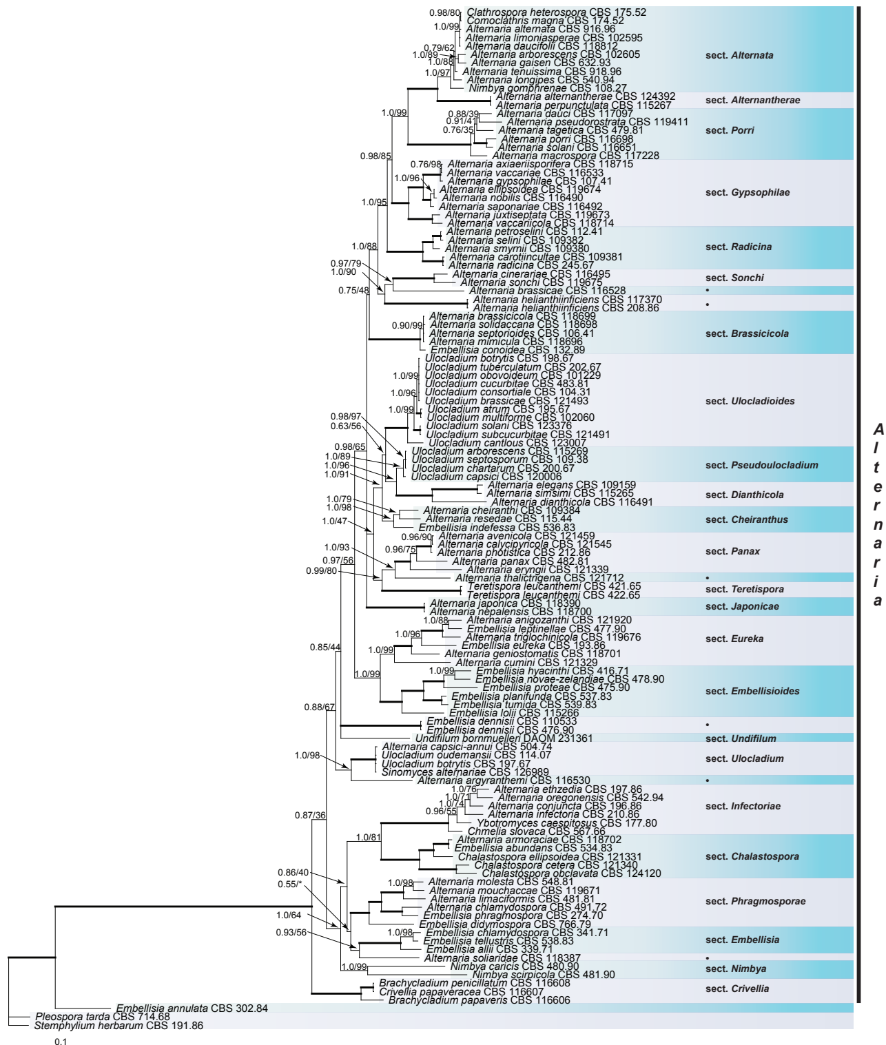
Fig. 1. Bayesian 50 % majority rule consensus tree based on the GAPDH, RPB2 and TEF1 sequences of 121 strains representing the Alternaria complex. The Bayesian posterior probabilities (PP) and RAXML bootstrap support values (ML) are given at the nodes (PP/ML). Thickened lines indicate a PP of 1.0 and ML of 100. The tree was rooted to Stemphylium herbarum (CBS 191.86). The monotypic lineages are indicated by black dots.
