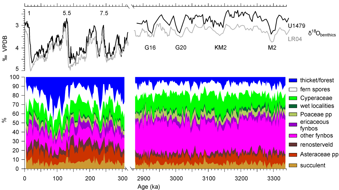
Figure 9. Summary diagram of the Pleistocene (left) and the Pliocene (right) pollen record of Site U1479. Note the larger fluctuations in the Pleistocene and compared to the Pliocene the strong increase of pollen from thicket/forest (mainly Podocarpaceae), increase in Asteraceae pp, a slight increase in succulent elements, and decline in other Fynbos pollen types (mainly Restionaceae). Pollen groups are listed in Table 4.
