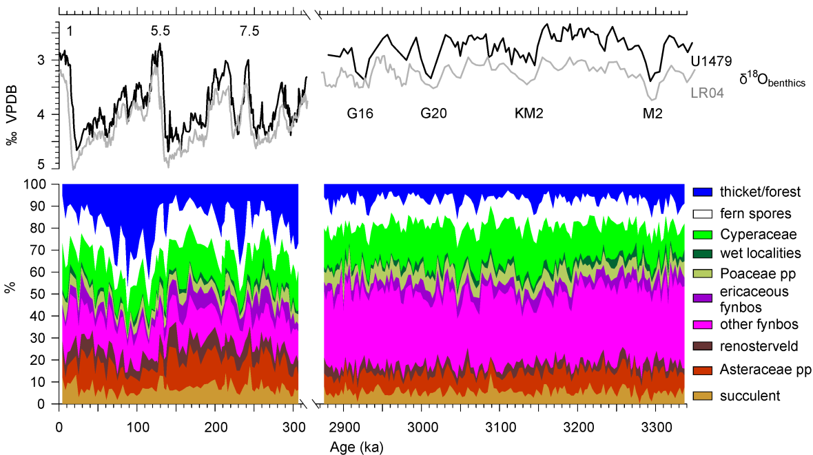
515 Figure 9. Summary diagram of the Pleistocene (left) and the Pliocene (right) pollen record of Site U1479. Note the larger fluctuations in the Pleistocene and the strong increase of thicket/forest (mainly Podocarpaceae) pollen, increase in Asteraceae pp pollen, a slight increase in succulent pollen, and decline in other Fynbos (mainly Restionaceae) pollen compared to the Pliocene. Pollen groups are listed in Table 4.
