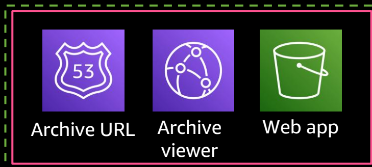
Web application
