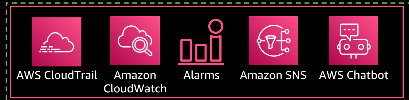
Monitoring
