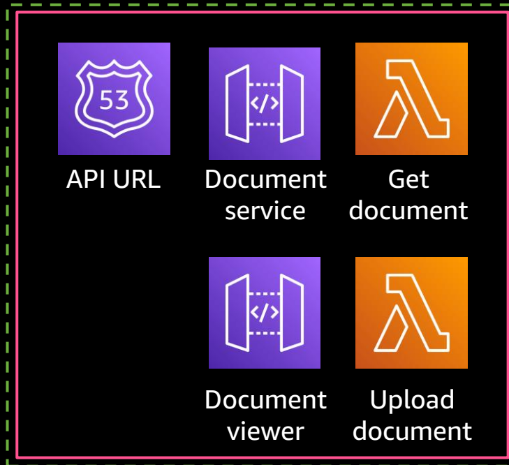
Document service
