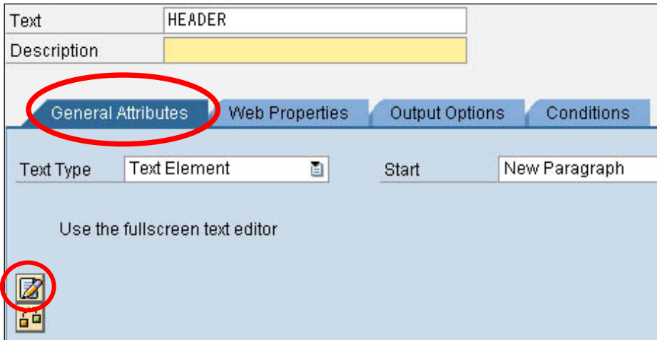
Figure 46 Adding Text
