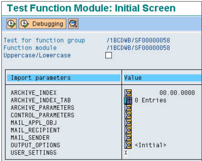
Figure 54 Printing Screen
