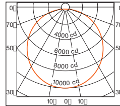
Polar diagram
