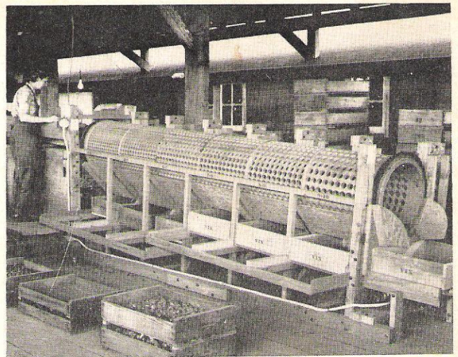
Iris Grader. Sizing the commercial bulbs, removing planting stock, cleaning and fanning; all in one operation.
