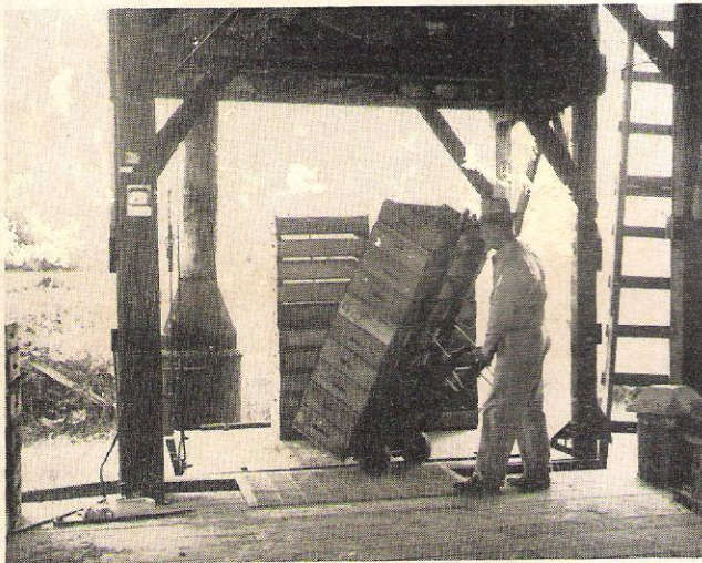
Loading Daffodils on a platform which is lowered into a sterilizing tank.
