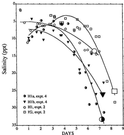
Figure 6.3. Sicydium spp. larvae Mean salinity exposure in each of four halocline (three H1 and one H2) treatments over time. Note inverted y axis scale. Lowercase a or b distinguish similar treatments in same experiment. Ages are days since either hatch (expt. 2) or capture (expt. 4). Large symbols identify curves. Maximum salinity available in H1 of expt. 3 was approximately 16 ppt. Adjusted r^2 range 0.67 to 0.89; p \leq 0.0001 for all.
