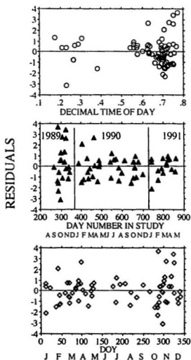
Figure 3.2. Residuals of regression (eq. 1) of \log_e goby larvae \cdot m^{-3} Against (upper to lower) time of day, day number in study, and DOY (see text).
