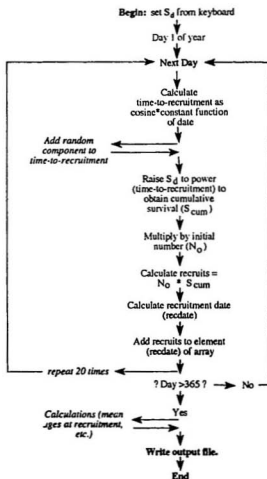
Figure 9.4. Flowchart for simulation, showing steps taken by the simulation program. Greyed arrows and italicised text on the left indicate additional steps which can incorporate individual variation into the model.
