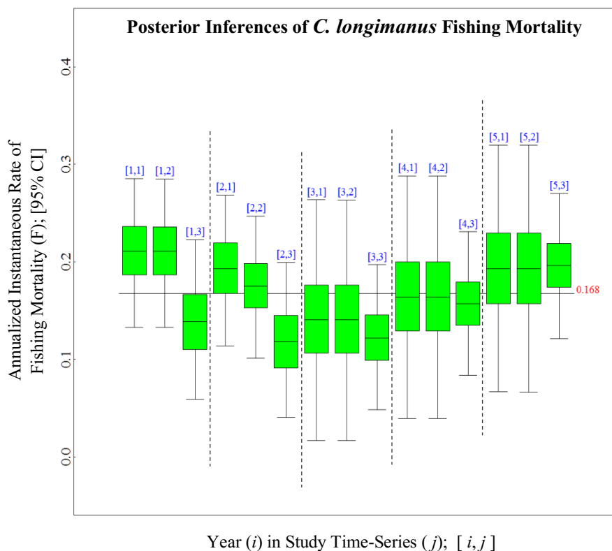
Figure A3-1a. Box Plots of Posterior Inferences of Carcharhinus longimanus Fishing Mortality by Year ( i ) and Individual Study Time-series ( j ) [2010-'14]. Dotted-lines organize groups of inferences in relation to their corresponding applicable year of output, and not by any data-set affiliation. [Indices: i = 1,...,5 is year 2010,...,2014; j = 1 is Abdussamad et al. (2012a & 2012b); j = 2 is Hornby et al. , (2015a & 2015b); j = 3 is India's National Reports to the Scientific Committee of the IOTC by the Fisheries Survey of India (Various Authors, 2010-2015)].
