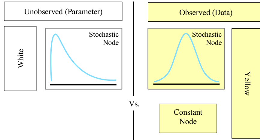
Figure 21d. Node color categorization (white vs. yellow). Distribution types (shapes) of stochastic nodes are arbitrary.
