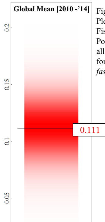
Figure A3–8b. Box Plots of Posterior Inferences of Mean Year-wise Fishing Mortality for Stegostoma fasciatum [2010-'14]; [ i = 1 is 2010, i = 2 is 2011, etc.].
