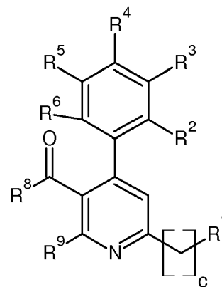
Formula (II),
