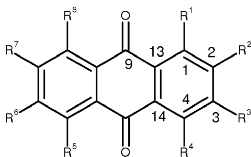
Formula (IIIId)
