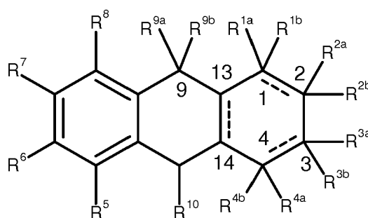
Formula (IIIb)
