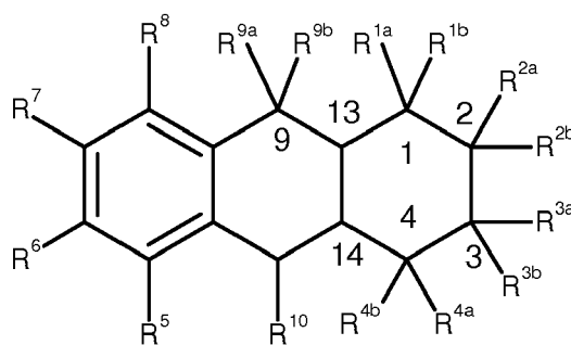
Formula (IIIc)
