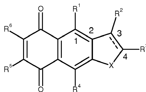
Formula (IV)
