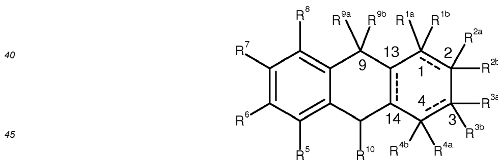
Formula (IIIb)
