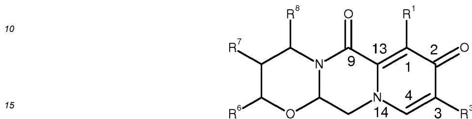
Formula (IIIa)
