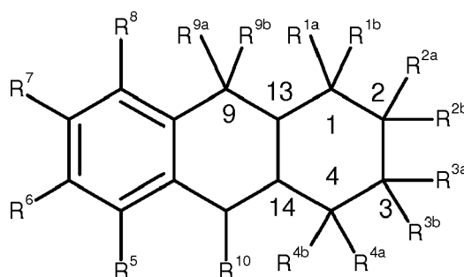
Formula (IIIc)
