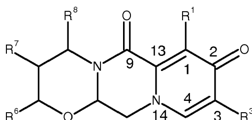
Formula (IIIa)
