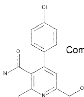
4-(4-chlorophenyl)-6-(hydroxymethyl)-2-methyl-pyridine-3-carboxamide
