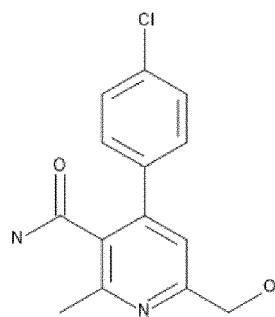
Compound-10
