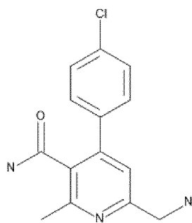
Compound-7
