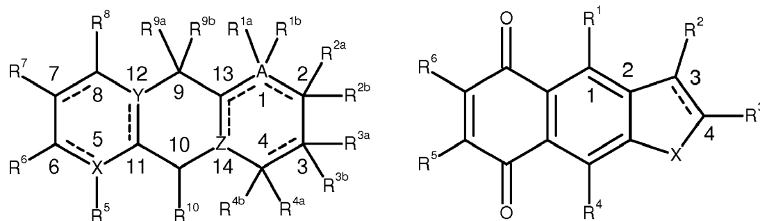
Formula (III)
