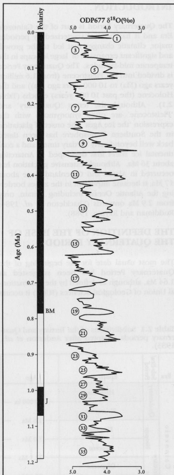
Figure 2.2 Oxygen isotope record and polarity from Ocean Drilling Program (ODP) site 677 (after Shackleton et al. , 1990). Normal polarity is indicated by black, reverse by white. No.s 1–35 are Oxygen Isotope Stages (OIS). BM: Brunhes–Matuyama boundary; J: Jaramillo event.
