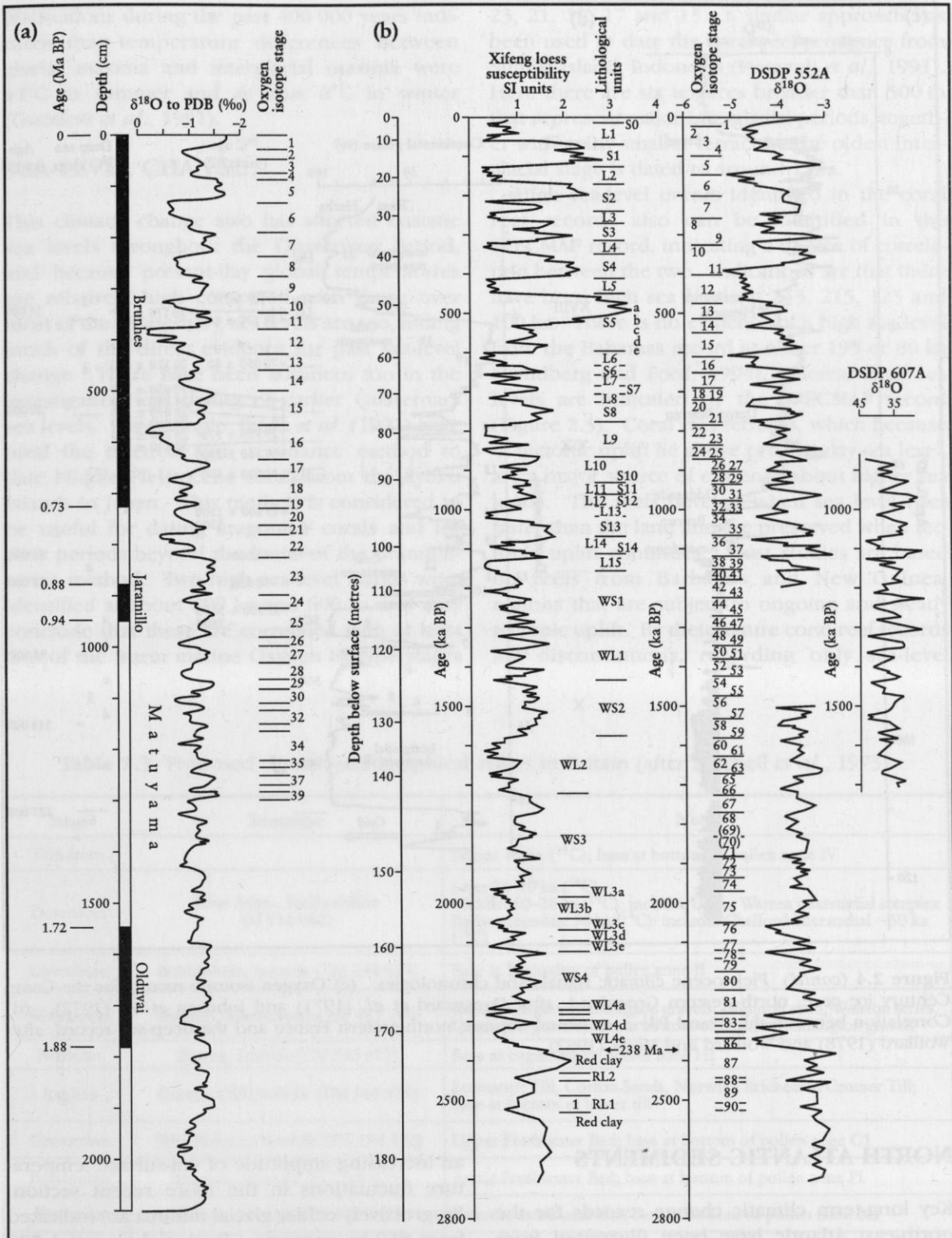
Figure 2.4 Pleistocene climatic signals and chronologies. (a) Oxygen isotope and palaeomagnetic record in core V28-239, after Shackleton and Opdyke (1976) and Berggren et al. (1980) PDB: Pee Dee Belemnite. (b) Magnetic susceptibility record in the Xifeng Loess and proposed correlation of the Chinese loess and soil units with the Oxygen Isotope Stages in the core 552A (Deep Sea Drilling Project), after Shackleton et al. (1984), Ruddiman et al. (1986) and Kukla (1987). See overleaf for (c) and (d).
