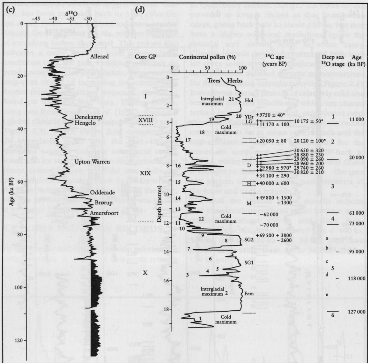
Figure 2.4 (cont'd) Pleistocene climatic signals and chronologies. (c) Oxygen isotope record for the Camp Century ice core, north-western Greenland, after Dansgaard et al. (1971) and Johnsen et al. (1972). (d) Correlation between the Grand Pile continental deposit, north-eastern France and the deep-sea record, after Woillard (1978) and Woillard and Mook (1982).
