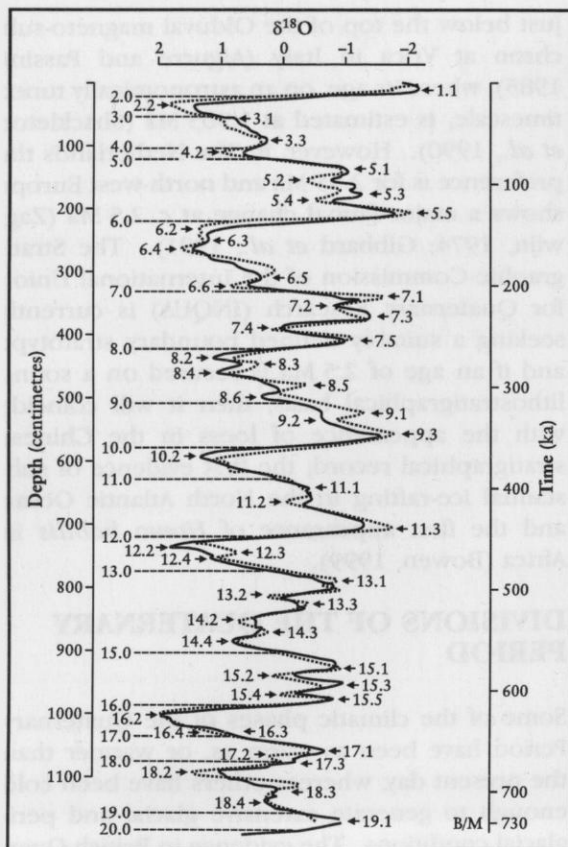
Figure 2.1 Oxygen isotope stratigraphy (after Prell et al. , 1986). A deep-sea core shows the variation of oxygen isotopes with depth (arbitrary units) and time (ka). Fluctuations to the left correspond to larger ice volumes on land (glacials) and conversely fluctuations to the right to reduced on-land ice, corresponding to interglacials. Curves represent different benthic foraminifera.
