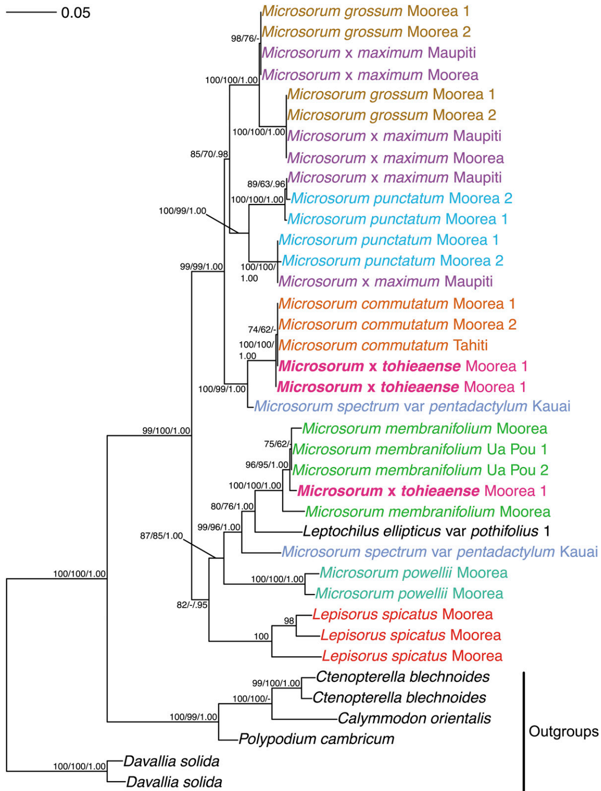
FIG. 5. Maximum-likelihood phylogenetic tree inferred using nuclear gapCp short including Society Islands microsoroid ferns and related taxa. Taxa occurring in Society Islands and Hawaii colored by taxon; taxa not occurring in these areas and outgroups in black. Microsorium x tohieaense in bold. Maximum likelihood bootstrap (MLBS), maximum parsimony bootstrap (MPBS), and Bayesian inference posterior probability (BIPP) values shown at nodes separated by slashes; values less than 50% (MLBS, MPBS) or 0.5 (BIPP) indicated with dash. Extremely short branchlengths ( < 1 \times 10^{-5} substitutions per site) have been collapsed to zero. Scalebar indicates substitutions per site.
