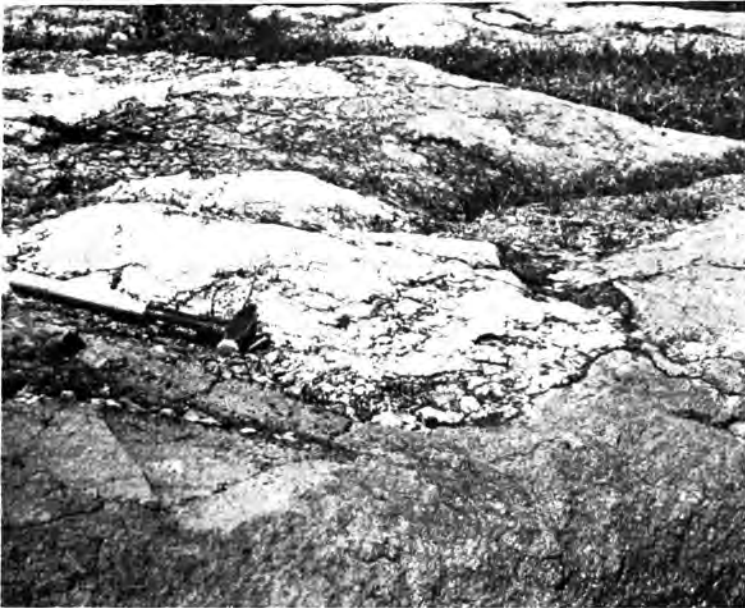
FIGURE 22. Reef rock (light areas) and flanking calcarenites (darker areas) in basal Valcour Limestone at abandoned quarry on Bechard Farm, west of Kings Bay
