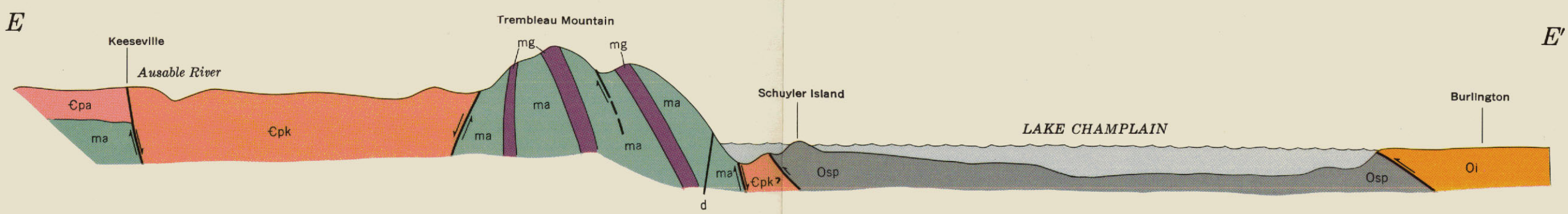
BEDROCK GEOLOGY OF THE PLATTSBURGH AND ROUSES POINT QUADRANGLES, NEW YORK AND VERMONT (PLATE 2)
