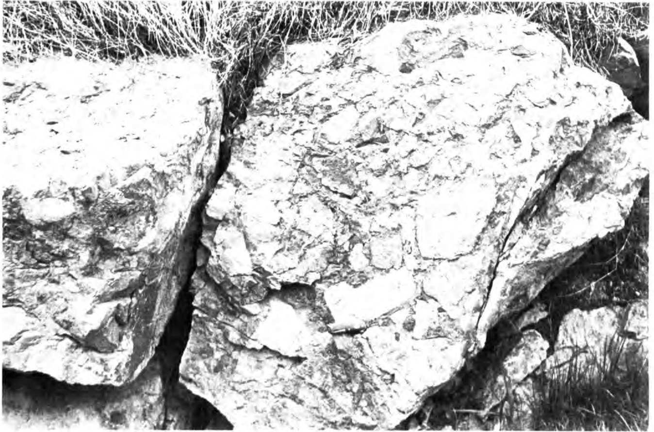
FIGURE 30. Fault breccia along Tracy Brook Fault, on west side of U.S. 9, north of railroad underpass in village of Chazy. The rock is entirely crushed Potsdam (Keeseville) Sandstone
