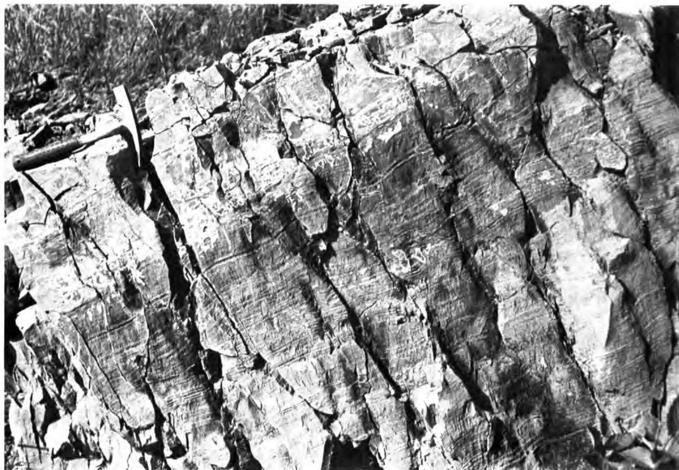
FIGURE 27. Bedding (dipping to left) and cleavage (dipping steeper to the right) in Cumberland Head Argillite, along U.S. 9, 4 miles north of Plattsburgh
