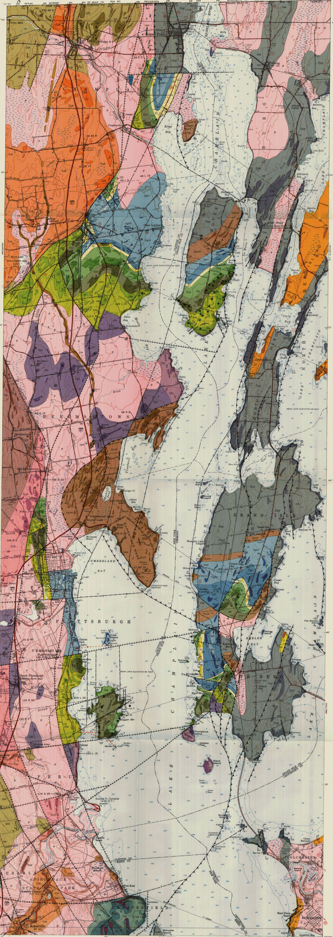
BEDROCK GEOLOGY OF THE PLATTSBURGH AND ROUSES POINT QUADRANGLES, NEW YORK AND VERMONT Base from quadrangles by the U.S.G.S. Scale 1:62,500 CONTOUR INTERVAL 20 FEET DATUM IS MEAN SEA LEVEL DEPTH CURVES AND SOUNDINGS IN FEET—DATUM IS MEAN LOW LAKE LEVEL 92.5 FEET APPROXIMATE MEAN DECLINATION, 1956
