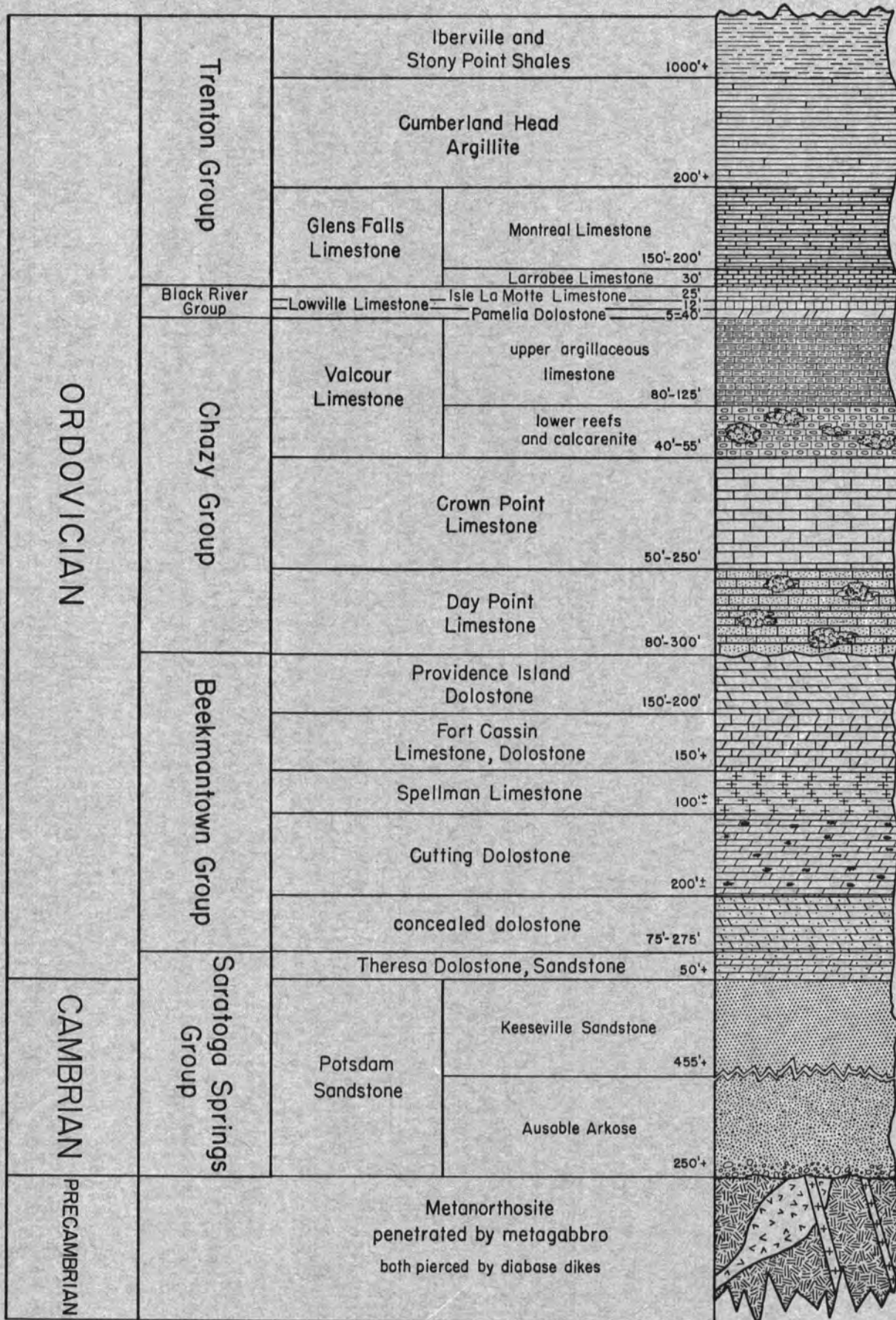
Figure 37 ROCK SECTION Plattsburgh and Rouses Point Quadrangles
