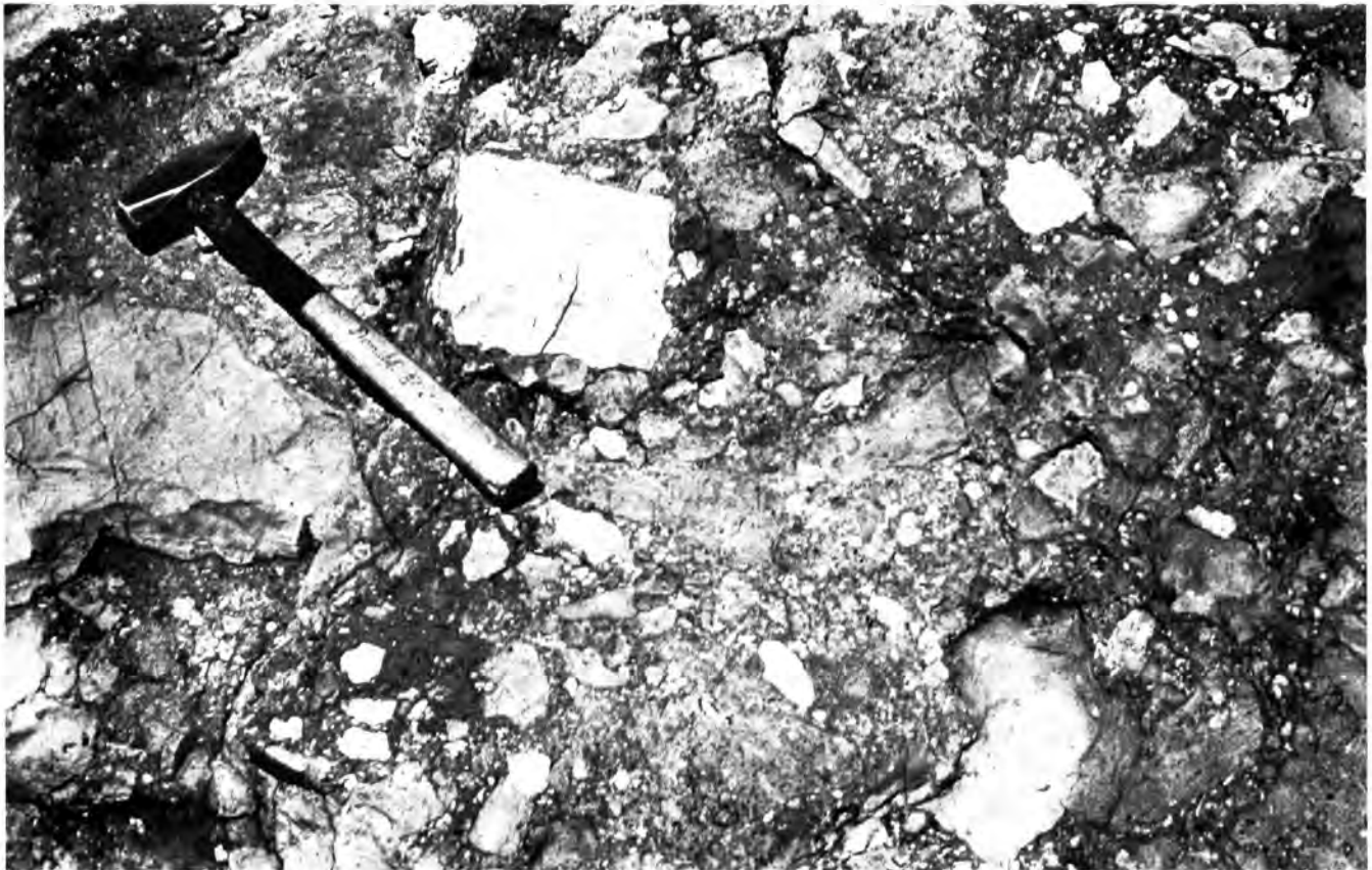
FIGURE 29. Lacolle Mélange , along south side of N.Y. 9A east of Coopersville. Note angularity and disparity in size of varied rock fragments
