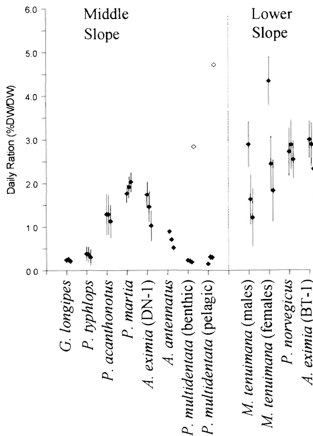
Fig. 3. Daily rations (% DW/DW) of decapod species studied arranged according to relative mobility (CL/CW ratio) for the middle-slope and lower-slope samples. (◊) Daily ration estimates obtained by direct analysis of stomach contents in Pasiphaea multidentata
