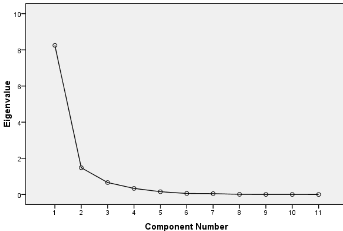
Correlation Matrix
