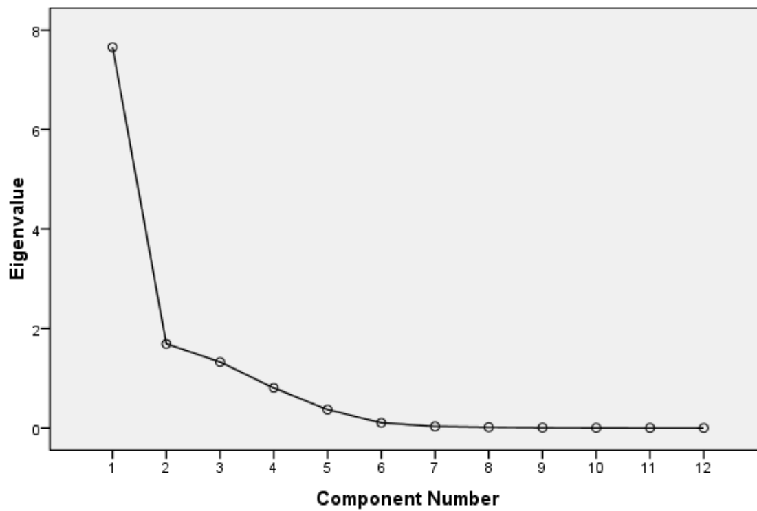
Scree Plot
