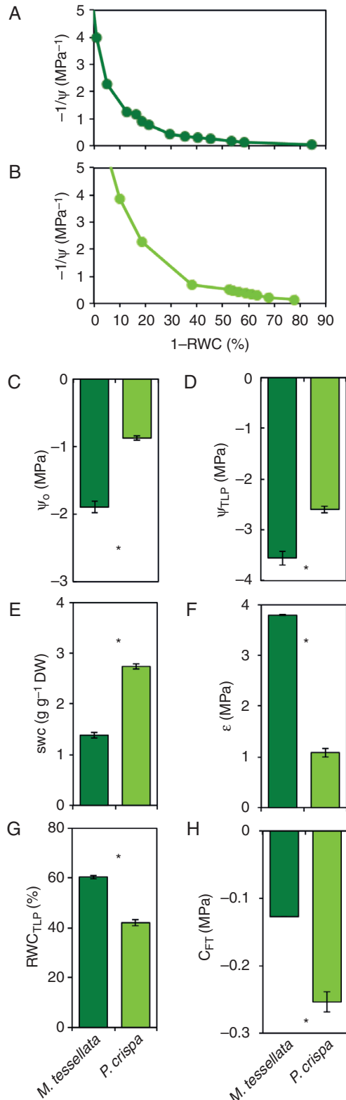
FIG. 5. (A, B) Pressure–volume (P–V) curves of thalli from M. tessellata (A) and P. crispa (B), showing the changes in inverse water potential ( 1/\psi ) as a function of water loss from the thalli ( 1 - \text{RWC} ). One representative measurement is shown for each species. (C–H) Selected parameters estimated from the P–V curves (see Materials and methods section for details of the calculations): water potential at full turgor ( \psi_0 ), water potential at the turgor loss point ( \psi_{TLP} ), symplastic water content at full turgor (SWC), modulus of elasticity ( \epsilon ), relative water content at turgor loss point ( \text{RWC}_{TLP} ) and capacitance before turgor loss ( C_{FT} ). Data are mean \pm s.e. ( n = 3 , for P. crispa , 2 for M. tessellata ). Asterisks denote significant differences among species at P < 0.05 .
