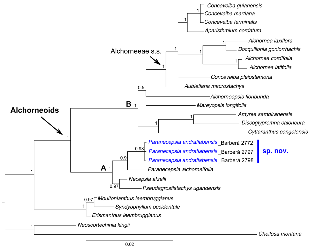
Fig. 1. Phylogenetic relationships of representatives of the alchorneoids clade within Euphorbiaceae-Acalyphoideae, including samples of the new species. Bayesian 50% majority-rule consensus tree based on the combined 2-marker, 26-tip dataset with posterior probability values indicated at nodes. Note: the name Conceveiba terminalis (Baill.) Müll.Arg. is used in place of Gavarretia terminalis Baill. in Wurdack et al. (2005).
