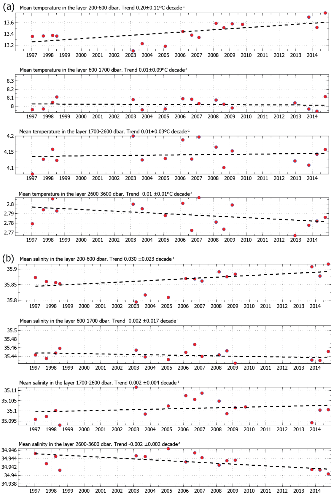
Figure 6.1.4. Time series of (a) mean temperature ( ^{\circ}\text{C} ) and (b) mean salinity between stations 11-24 for four different vertical strata, representative of the central waters (200-600 dbar), intermediate waters (600-1700 dbar), and deep waters (2600-3600 dbar). Trend (dashed line) and trend values, and statistical significant range at the 95% confidence level are indicated for each depth stratum.
