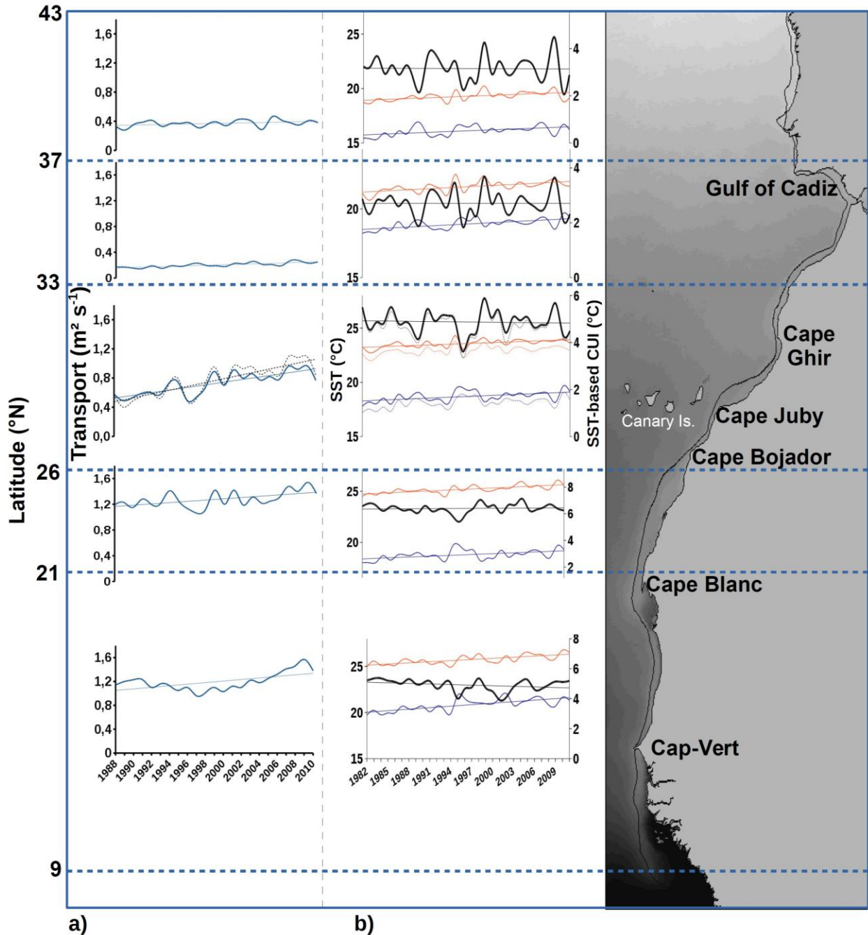
Figure 6.3.5. Linear trends for a) the annual-mean Ekman Transport ( \text{m}^2 \text{s}^{-1} ) during 1988-2011 for the five regions of upwelling regimes previously defined, and b) the annual-mean SST during 1982-2011 for \text{SST}_{\text{max}} (red line), \text{SST}_{\text{min}} (blue line) and CUI (thick black line). The Cape Ghir trends (dashed lines) are superimposed on the plot for the 26°N-33°N area.
