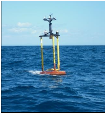
Figure 3.6.2. Left picture: Seawatch buoy from the Deep Water Network; Right picture: Triaxys buoy from the Coastal Network.
