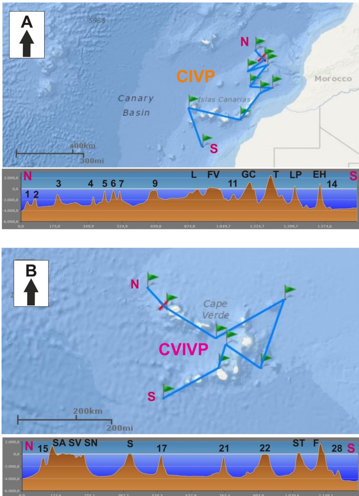
Figure 2.2.3. Bathymetric profiles on islands and seamounts of the CIVP (A) and CVIVP (B) (modified from Becker et al., 2009). Numbers refer to seamounts (see Tab. 2.2.1). Capital letters refer to island names (see Figs. 2.2.2 and 2.2.3)
