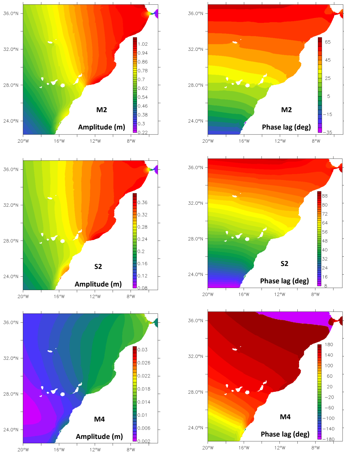
Figure 3.6.9. Spatial variation of amplitude and phase of M 2 , S 2 and M 4 harmonic constituents from the COMAPI tidal atlas in the area of interest (resolution 1'×1').
