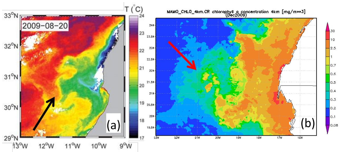
Figure 3.5.2. (a) Signature of the Cape Ghir filament on the SST field. (b) Signature of the Cape Blanc Giant filament on the chlorophyll-a field as obtained from MODIS aqua 4 km resolution data (Giovanni Ocean Color Radiometry Online Visualization and Analysis, http://gdata1.sci.gsfc.nasa.gov/daac-bin/G3/gui.cgi?instance_id=ocean_month , accessed 9 April 2015) for December 2009.
