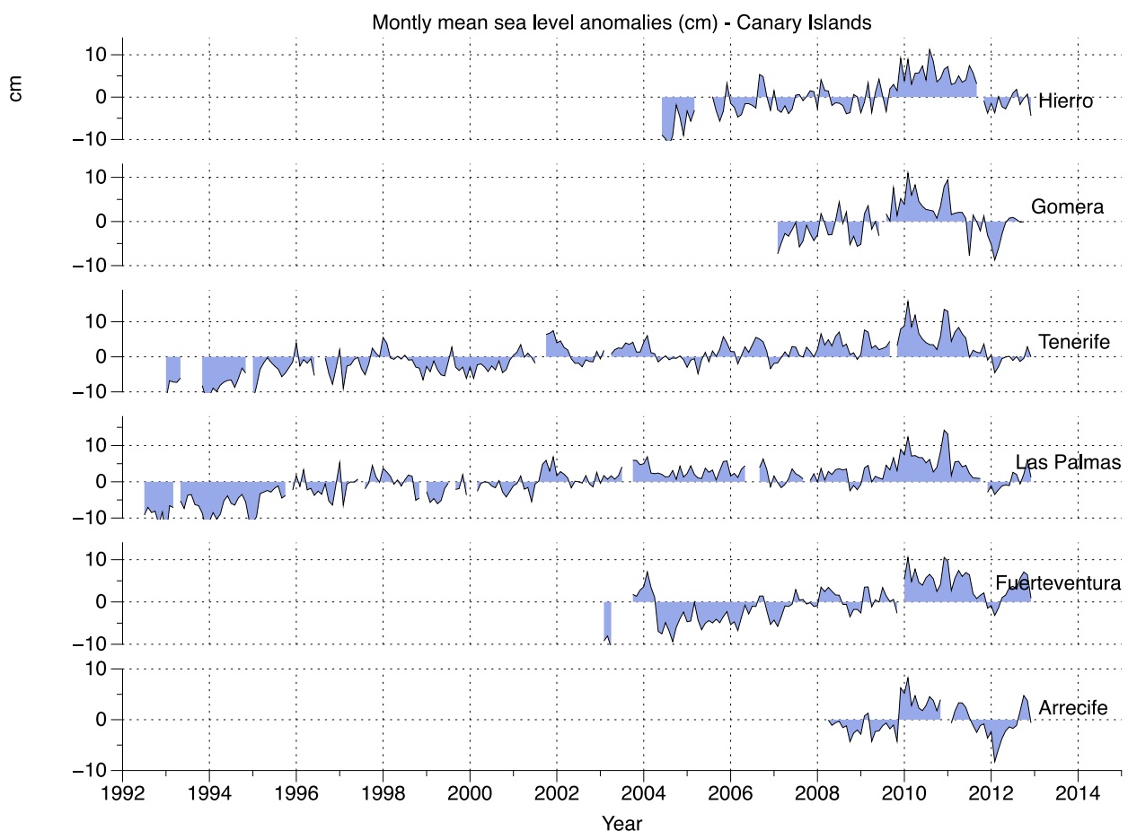
Figure 6.2.2. Monthly mean sea level anomalies at the REDMAR stations in the Canary Islands, since their start date of operation until 2012 (extracted from Pérez-Gómez, 2014).
