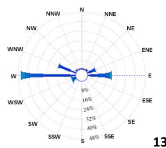
Figure 3.6.7. Wave roses of 13 model points representing different locations of the area of interest.
