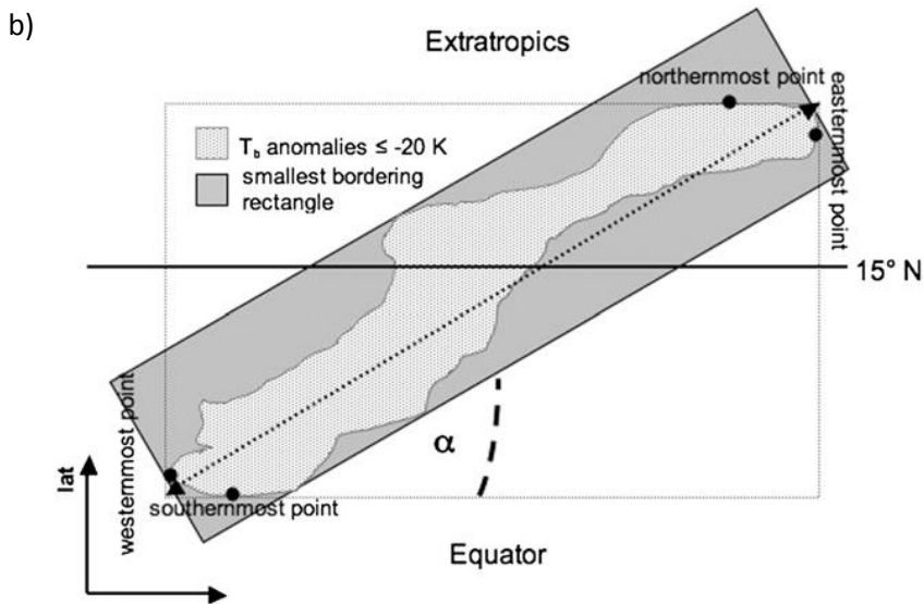
Figure 3.1.4. a) Satellite MET10 infrared imagery at 15:00 UTC 11 Apr 2015 showing the development of a tropical plume over the NWA extending from Cabo Verde to Western Sahara, Mauritania, and Algeria (Source: EUMETSAT, website at http://oiswww.eumetsat.org/PPS/html/MSG/PRODUCTS/MP E/WESTERNAFRICA/index.htm , accessed on 12 April 2015). b) Schematic illustration of the TP identification procedure for the Northern Hemisphere (reproduced from Fröhlich et al., 2013). The inclination angle ( \alpha ) between the SW NE direction of the elongated clouds centered at latitude 15^{\circ}\text{N} and the Equator. The grey and light grey correspond to the inclined rectangle range that of the clouds and the temperature anomalies less than or equal to 20\text{ K} . © American Meteorological Society.
