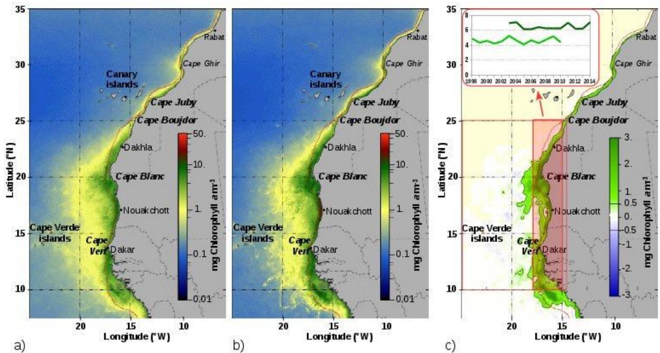
Figure 6.4.1. Average chlorophyll-a concentrations from a) SeaWiFS and b) MODIS data from 2003 to 2007 and c) the MODIS-SeaWiFS difference for the same period. The 200 m depth contour (red line) is superimposed. The insert in plot (c) shows the yearly averages of both sensors from 1998 to 2014 in the coastal area as defined by the red rectangle.
