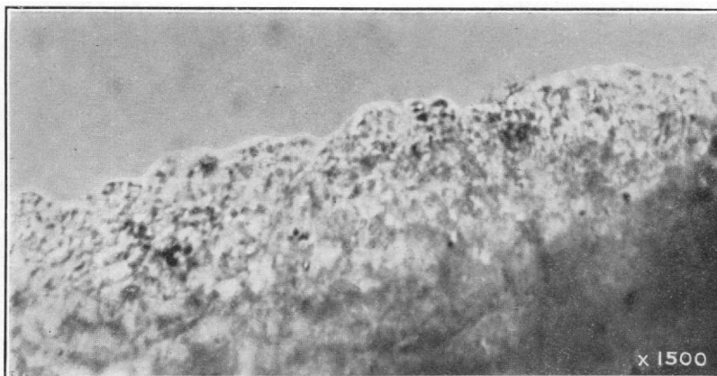
A. A PORTION OF A GROUND VERTICAL SECTION OF THE BLACK CRUST ILLUSTRATED IN B
