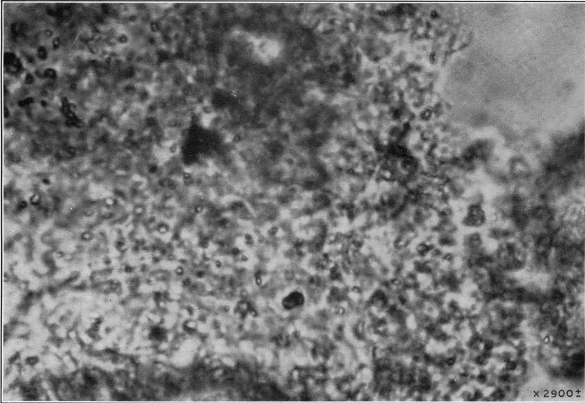
A. LITHOMYXA CALCIGENA , DECALCIFIED, MORE OR LESS EMBEDDED IN COLLOIDAL JELLY, FROM SURFACE LAYER OF A CALCAREOUS PEBBLE, FURNACE CREEK, W. VA. Collected by White, Howe, and Read December 7, 1930.
