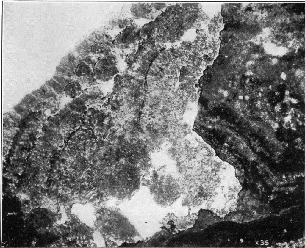
B. A GROUND SECTION AT THE LINE OF JUNCTURE OF THE GRAY TRAVERTINE AND THE BLACK. The Lyngbya and Inactis form the looser and (in section) flabellate crusts at the left. The Lithomyza forms the more compact and homogeneous crust at the right.
