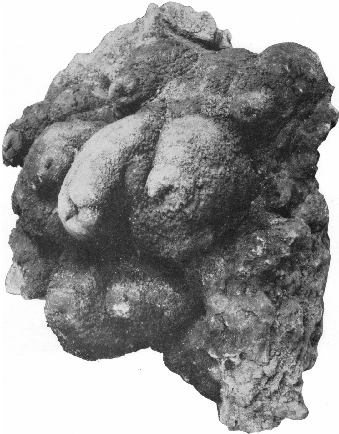
CALCAREOUS TRAVERTINE FORMED CHIEFLY BY LITHOMYXA CALCIGENA FORM FERRIFERA , IN MORE OR LESS SHADED PLACES IN RAPIDLY MOVING WATER, FURNACE CREEK, W. VA.
