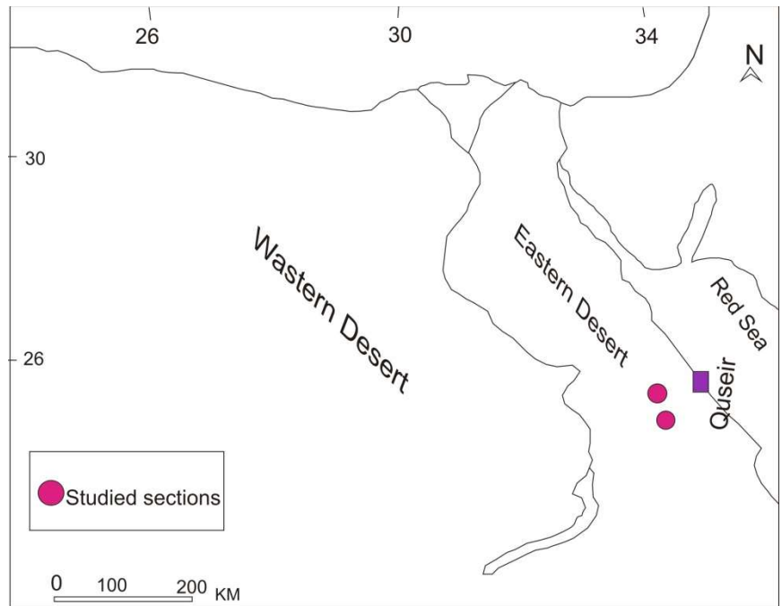
Fig 1. Location map of the studied sections(Gebel El Duwi &Gebel Atshan).
