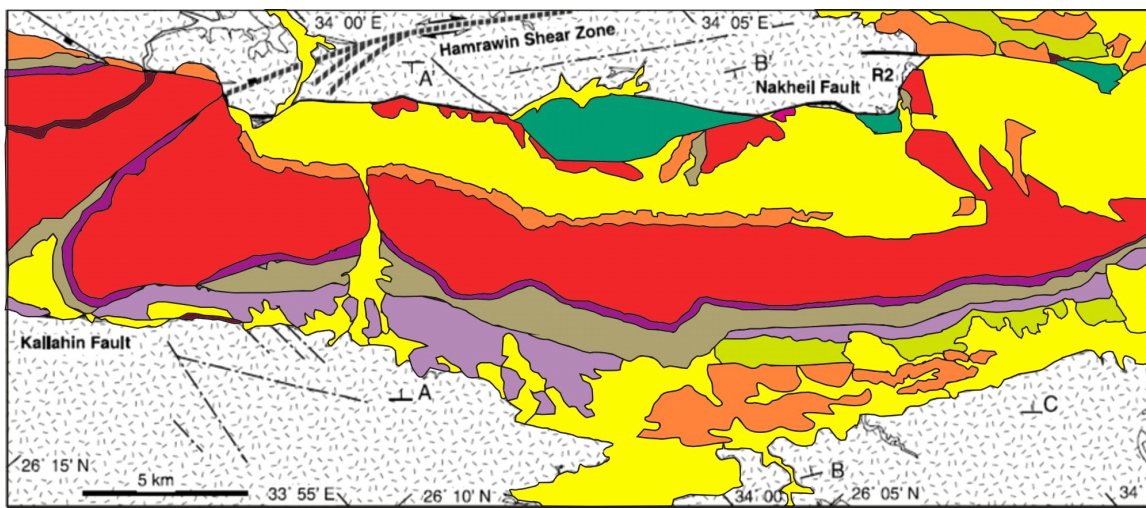
Fig . 2. Geologic map of the studied area, modified after Khalil& Meclay (2002).
