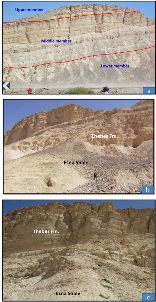
Fig. 6. a- Three informal members of the Thebes formation at Gebel Atshan Section, b- Esna Shale and Thebes Formations at Gebel Atshan, c, Gradational contact between Esna and Thebes formations at Gebel Atshan Section.
