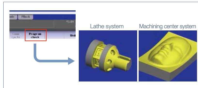
A click of the menu button navigates you to 3D graphic check of the currently edited program. For lathe system, the 3D check supports for both milling and turning.
