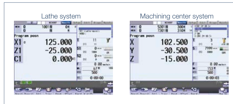
Simple screen with narrowed-down information is easy to see from a distance.
