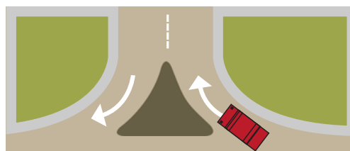
FIGURE 7.4.102 Right-in / Right-out
