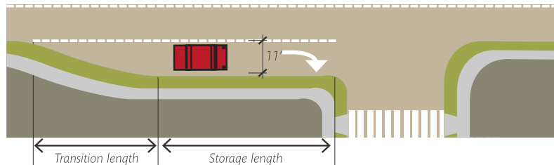
FIGURE 7.4.100 Right-turn Lane Design Elements
