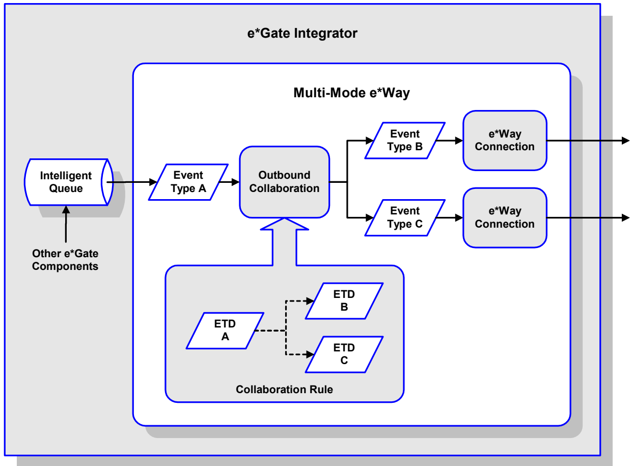
Figure 104 Outbound Collaboration
