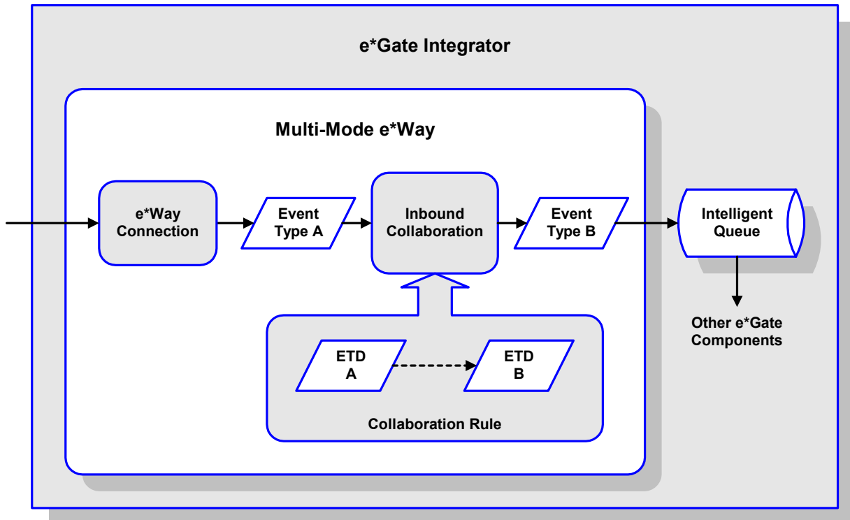
Figure 103 Inbound Collaboration
