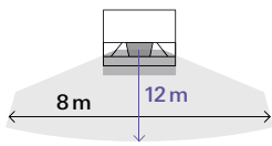
Busch-Watchdog 70 MasterLINE.
