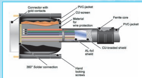
[3] ROLINE High Quality Monitor Cable with ferrite
