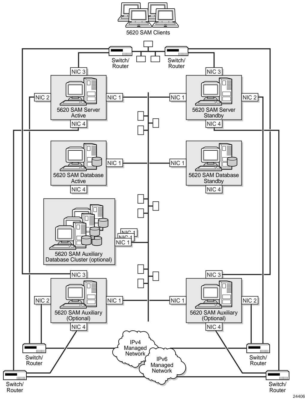
Figure 8-2 Distributed 5620 SAM Server/Database deployment with multiple network interfaces
