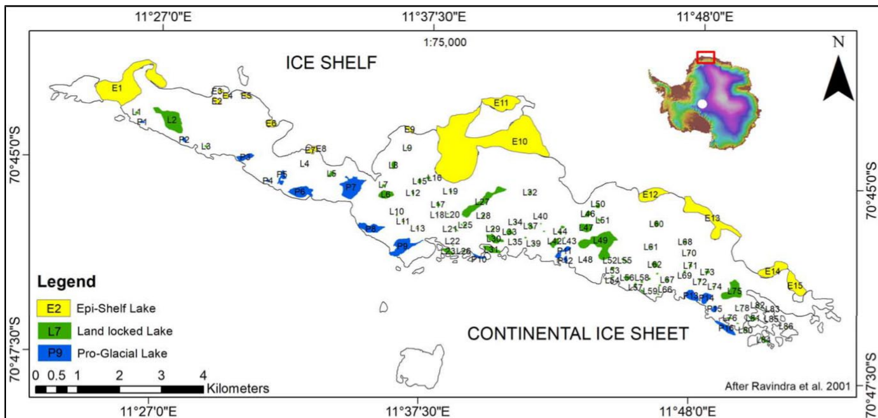
MAP 3: CLASSIFICATION AND NUMBERING OF LAKES, SHIRMACHER HILLS
