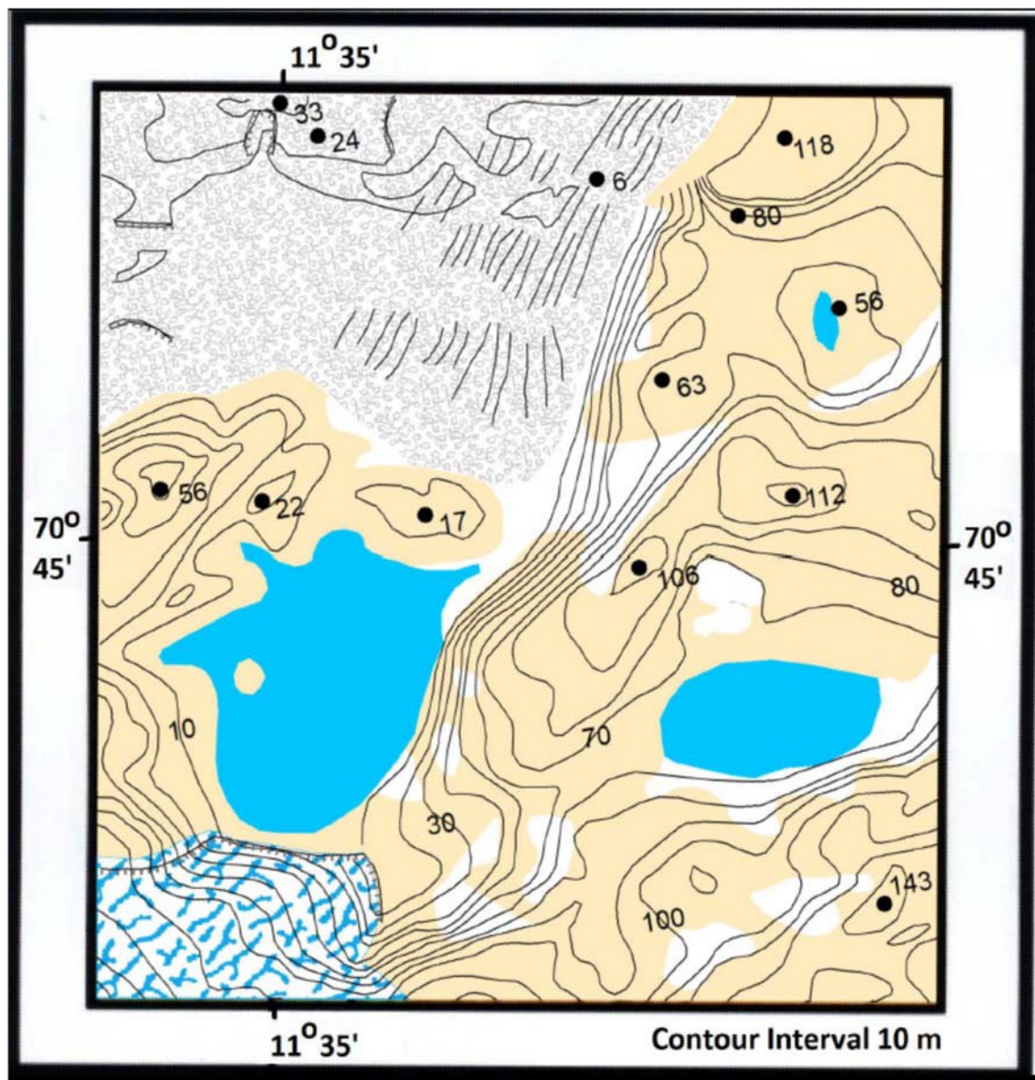
MAP 4: TOPOGRAPHIC MAP OF THE AREA
