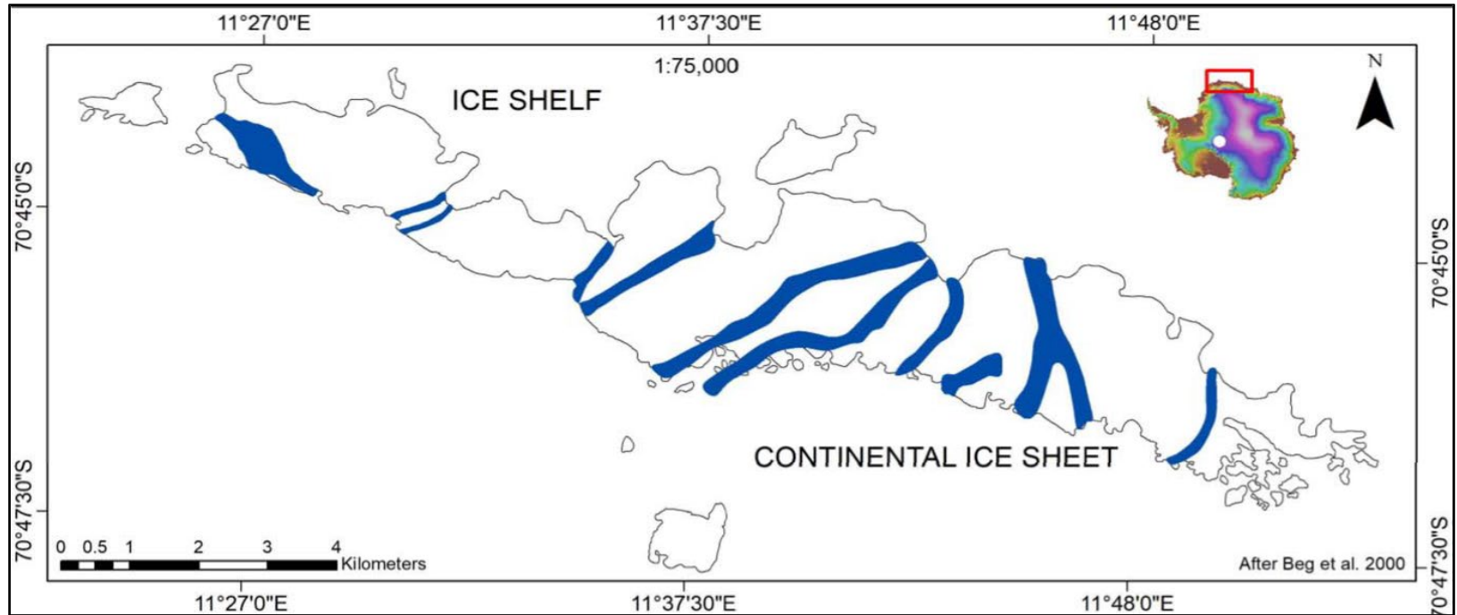
MAP 5: PATHS OF FOSSIL GLACIERS IN SCHIRMACHER HILLS
