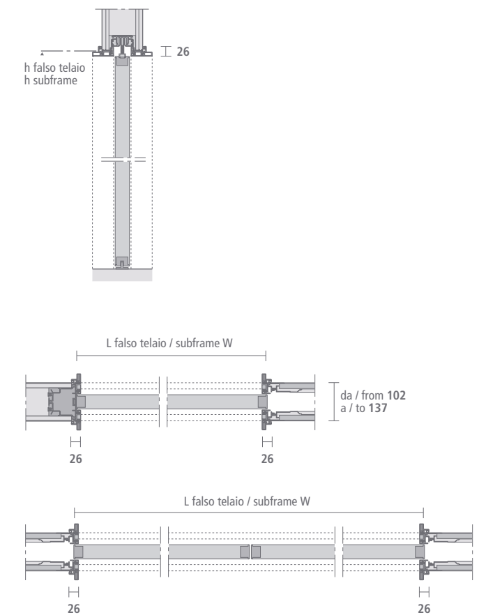
Slim Porta scorrevole per controlelai Scigno® Essential e Eclisse® Syntesis® line Pocket door for systems "Essential" by Scigno® and "Syntesis® line" by Eclisse
