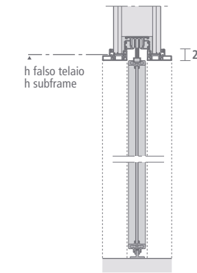
Slim Porta scorrevole per controlelai Scigno® Essential e Eclisse® Syntesis® line Pocket door for systems "Essential" by Scigno® and "Syntesis® line" by Eclisse
