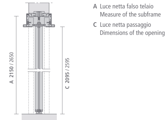
Porta scorrevole per controlelai a scomparsa Sliding door in the wall
