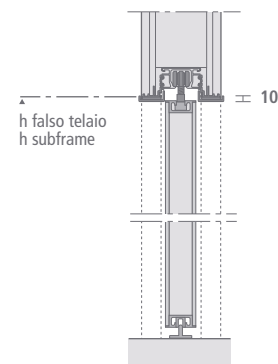
Porta scorrevole per controtelai Scigno® Essential e Eclisse® Syntesis® line Pocket door for systems "Essential" by Scigno® and "Syntesis® line" by Eclisse
