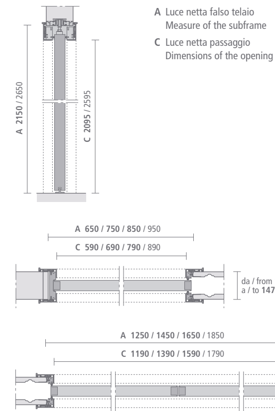
Porta scorrevole per controlelai a scomparsa Sliding door in the wall
