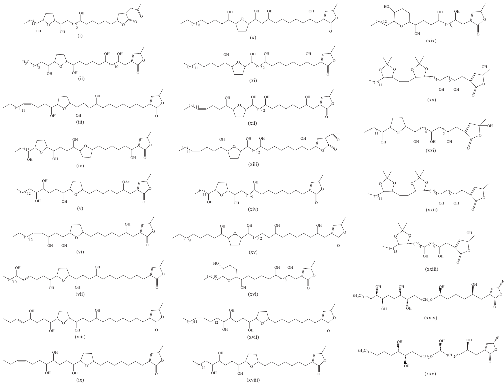
Figure 1. Acetogenins from Goniothalamus species.
