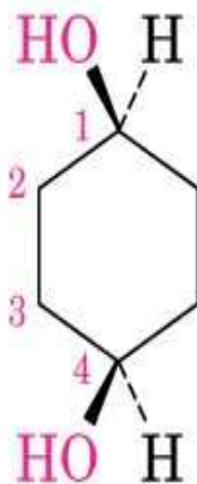
cis-1,4-Cyclohexanediol
