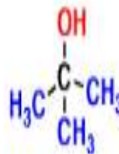
Tertiary Alcohol
