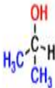
Secondary Alcohol
