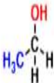
Primary alcohol
