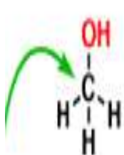
Methanol
