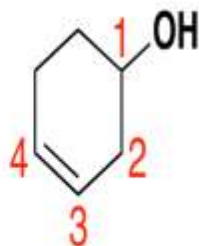
3-cyclohexen-1-ol
