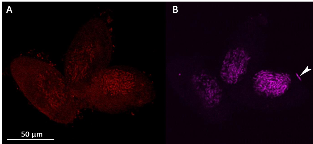
Figure 4 Cells of P. putrinum with symbionts in macronuclei labelled with the probes ALF1b (A) and Gyak567 (B). Single IF lying outside the macronucleus is shown with the white arrowhead.
