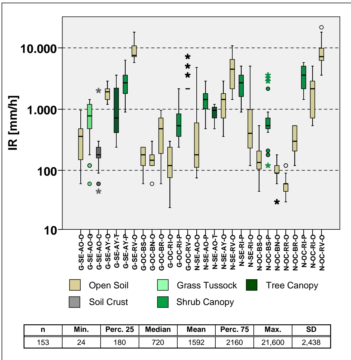
Fig. 5.14: Overview of single ring infiltration rates of different D4-units on the observatories Gellap and Nabaos.
