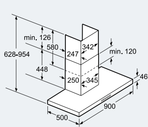
measurements in mm
