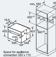
Space for appliance connection 320 x 115
