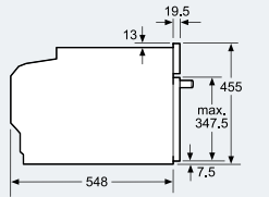
measurements in mm
