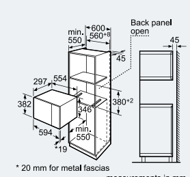
measurements in mm
