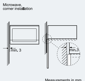
Measurements in mm
