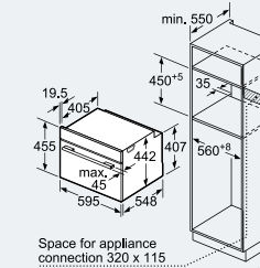
measurements in mm
