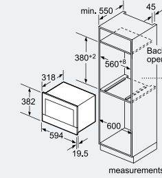
measurements in mm
