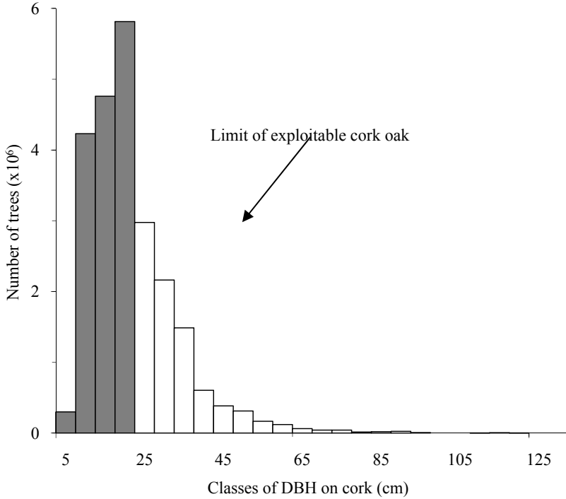
Figure 2. Number of cork oak trees related to the DBH on cork in Kroumirie forest (IFN 1995).
