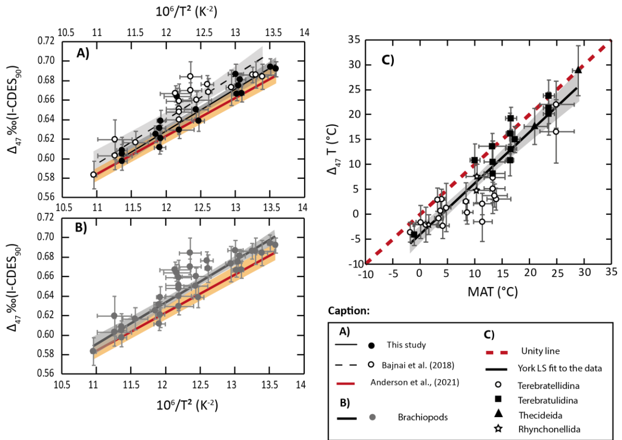
445 Figure 5: Comparison of \Delta_{47} values from modern brachiopods with the state-of-the-art \Delta_{47} calibration of Anderson et al., (2021). Envelope and error bars at 2\sigma . A. Comparison of York least square regressions (York et al., 2004) derived from two modern brachiopod datasets (Bajnai et al., 2018; this study) with the equation of Anderson et al., (2021). B. Comparison of York least square regression derived from the combined modern brachiopod dataset with the equation of Anderson et al., (2021). C) Comparison of modern brachiopods \Delta_{47} 450 temperatures calculated using the equation of Anderson et al., (2021) with seawater temperatures.
