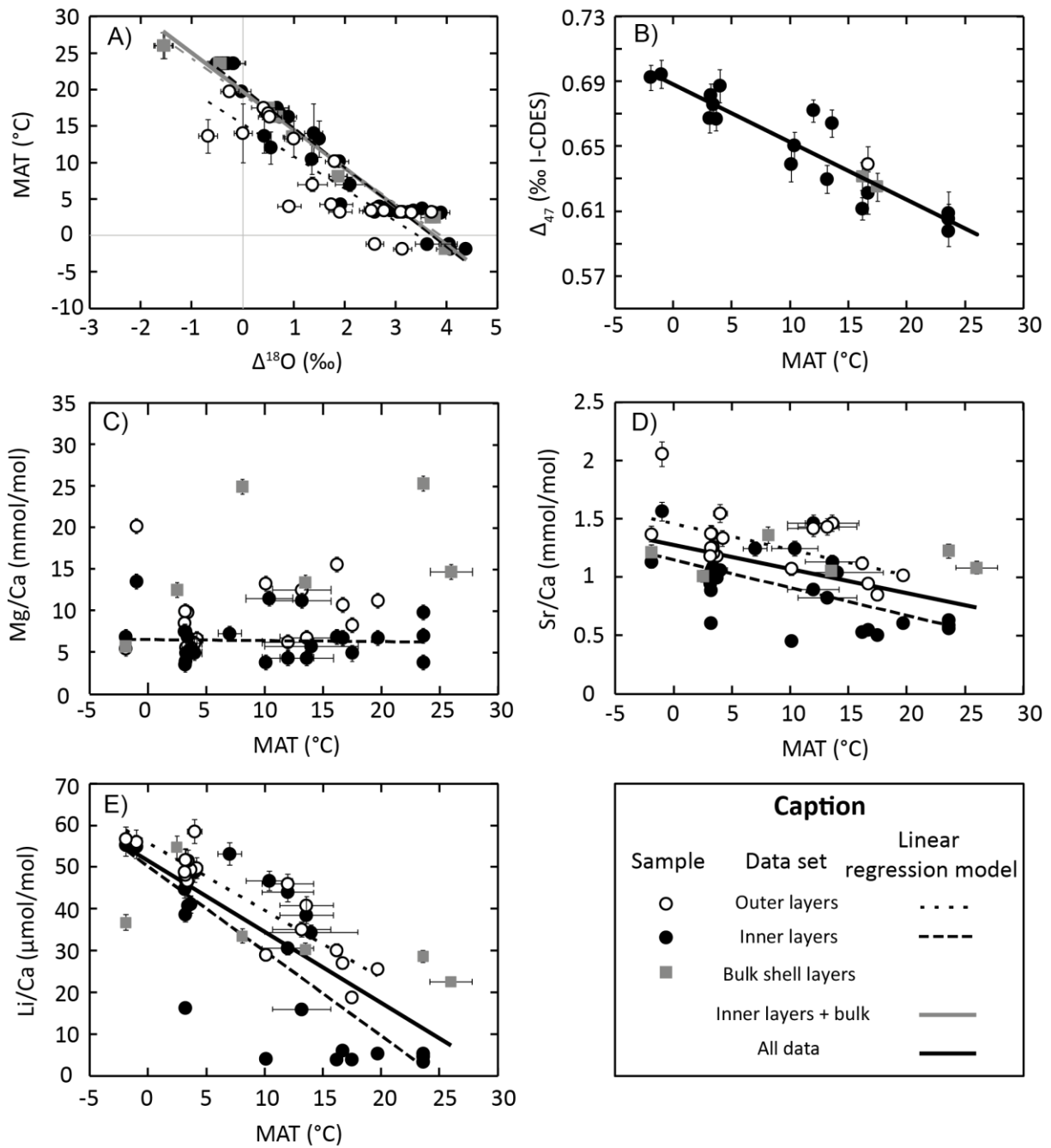
270 Figure 1: Geochemical data and linear regression model for each geochemical parameter tested for its relationship with brachiopod living temperature. Parameters associated with each regression model are listed in table 3.
