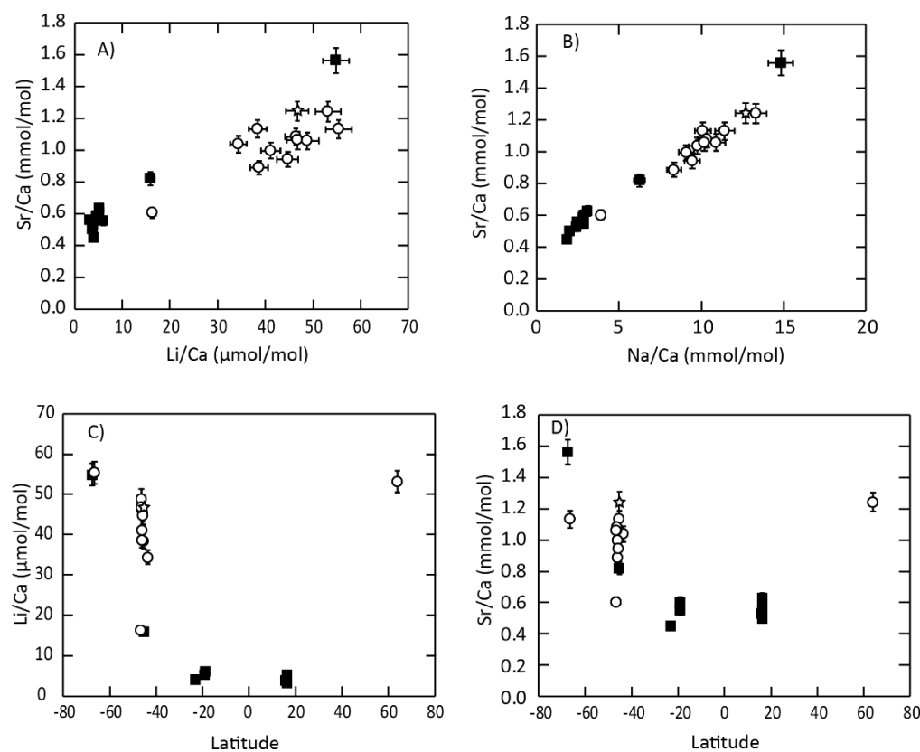
540 Figure 6: Distribution of trace element content of the inner shell layers among the different brachiopod taxonomic groups (Same symbols as in Figure 5C). The data show a strong correlation between Sr/Ca and Li/Ca (A) and Sr/Ca and Na/Ca (B), as well as strong latitudinal partitioning of Li/Ca (C) and Sr/Ca (D) values.
