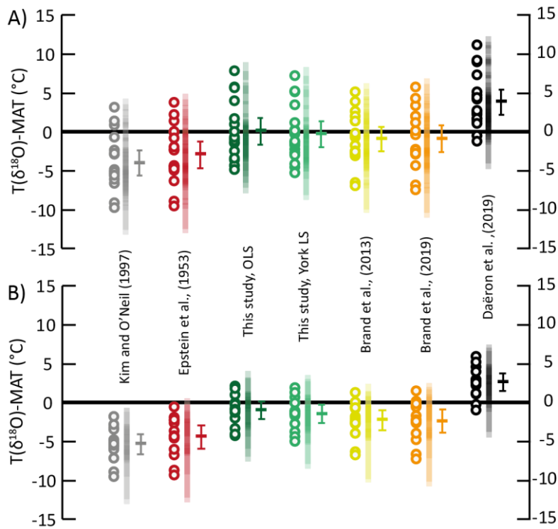
350 Figure 3: Offsets between the \delta^{18}\text{O} temperatures and MAT from the modern brachiopod dataset of Bajnai et al. (2018) using different fractionation equations. Circles: temperature offset for each sample; vertical transparent bars: temperature offset 95% confidence interval for each samples; horizontal bar: temperature offset arithmetic mean and associated 95% confidence interval of the mean. A) Temperature offset for isotopic temperatures calculated with \delta^{18}\text{O}_{\text{sw}} values calculated from the LeGrande and Schmidt (2006) database; N=18. B) Temperature 355 offset for isotopic temperatures calculated with locally measured \delta^{18}\text{O}_{\text{sw}} values; N=13. OLS = ordinary least square regression; YLS = York least square regression (York et al., 2004).
