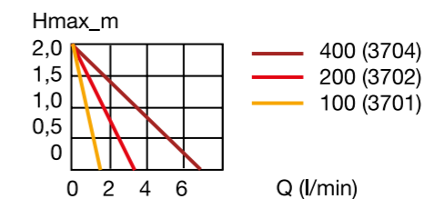
Air pump output diagram
