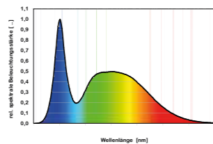
Colour spectrum powerLED+ fresh daylight
