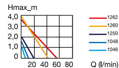
Universal pumps output diagram
