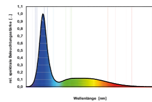
Colour spectrum powerLED+ marine hybrid
