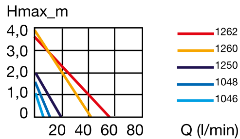
Universal pumps output diagram
