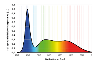
Colour spectrum powerLED+ fresh plants
