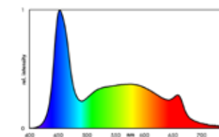
Colour spectrum classicLED plants
