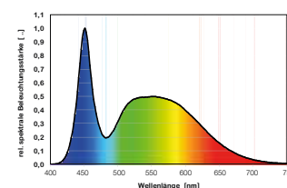
Colour spectrum powerLED+ fresh daylight
