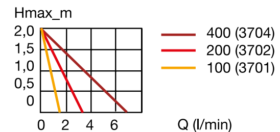
Air pump output diagram
