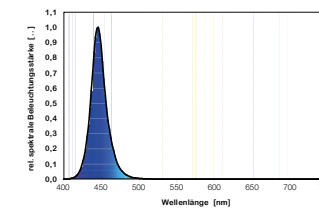
Colour spectrum powerLED+ marine actinic
