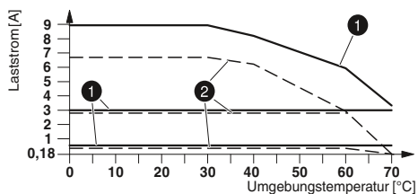
Derating-Kurve
