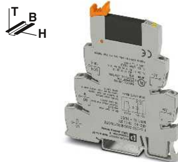
Solid-State-Relaismodul, DC-Ausgang max. 100 mA
