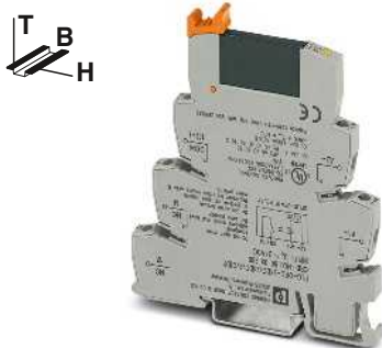
Solid-State-Relaismodul, DC-Ausgang max. 3 A
