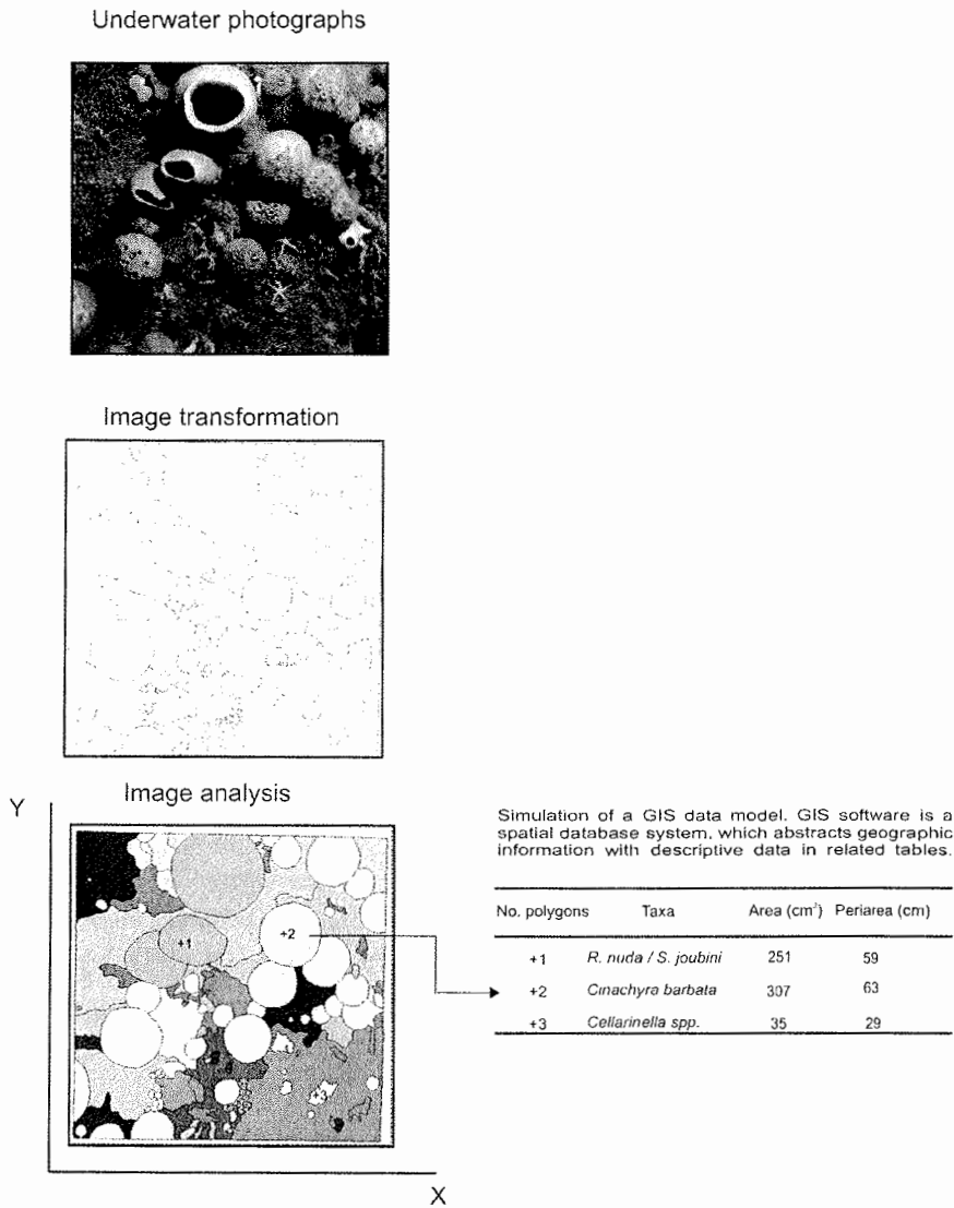
Fig. 6. From underwater photographs to vector computer images. Image transformation: the drawings were scanned and submitted to different technical processes (converted into black and white and the lines were thinned to unit width). Image analysis: the images were imported into Arc/View 3.2 (© ESRI) where they were georeferenced and labeled. Finally, the images were transformed to vector coverage data to calculate LPI using the program Fragstats v3.0 for Arc/Info (© ESRI).
