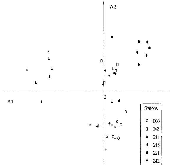
Fig. 8. Canonical variate analysis (CVA) defined by the two first axes (81 % of the total variability) based on LPI for the 6 stations. Each point corresponds to one photograph analysed. Indices included in the analysis: CA, MPS, PSSD, PSCV, NP, TE, MSI, AWMSI, LSI, PERIAREA, SHDI, SHEI, PR, and IJI.
