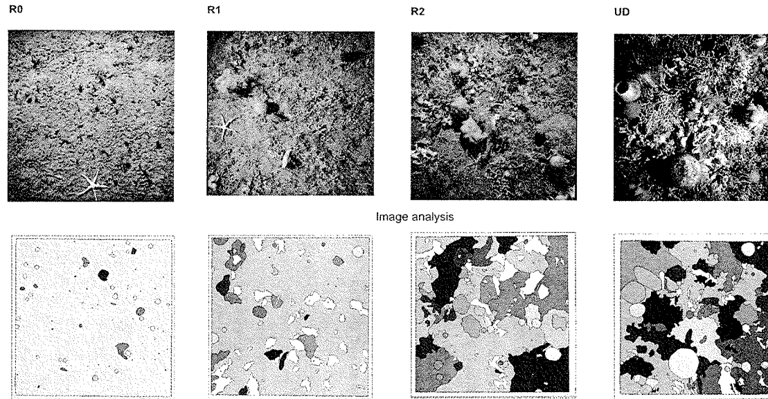
Fig. 2. Stages of recolonisation (from younger to older: R0, R1, R2) and undisturbed (UD) assemblage analysed. For each image, landscape pattern indices (LPI) were calculated using the program Fragstats v3.0 for Arc/Info. R0: Sediment surface is barely covered by sessile organisms such as lollypop like sponges ( Stylocordyla borealis ), soft bryozoans ( Camptoplites lewaldi and Bryozoa non identified), sabellid polychaetes ( Myxicola cf. sulcata ), and solitary ascidians ( Molgula pedunculata ). Large numbers of ophiuroids are also characteristic (the yellow sponge Iophon radiatus covers the surface of Ophiurolepis spp. ). R1: The yellow ( Cellarinella spp. and Systemopora contracta ) and white ( Hornea sp. ) rigid species of bryozoans, sabellid polychaetes ( M. cf. sulcata and Perkinsiana spp. ), and solitary ( M. pedunculata ) and colonial ascidians ( Distaplia cylindrica ) partially cover the seafloor. R2: Composed of a mixture of benthic organisms - round demosponges ( Cinachyra barbata ), a ramified-bushy gorgonian ( Notisis sp. ), soft ( Notoplites spp. ) and rigid bryozoans ( Cellarinella spp. and S. contracta , Reteporella spp. ), sabellid polychaetes, compound ascidians ( Aplidium sp.3 and Polysyncraton trivolutum ) and a pterobranchian ( Pterobranchia sp.2 ) -, which may cover up to three quarters of the area. UD: A volcano-shaped hexactinellid sponge ( Rossella nuda/ Scolymastra joubini ), a round demosponge ( C. barbata ), rigid ( Smitina directa , Cellarinella spp. ) and cigar-like bryozoans ( Smittoidea malleata ), a salmon "bottle brush" gorgonian ( Thouarella sp.2 ), a holothurian ( Ekmocucumis turqueti ), and compound ascidians ( Aplidium sp. 3 and Synicum adareanum ) cover the seafloor.
