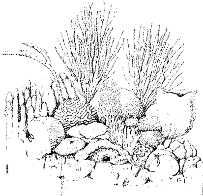
Fig. 16. Idealized diagram of a) Antarctic benthic shelf community, b) Mediterranean "coralligenous" benthic community, and c) coral reef benthic community. Representative species are indicated. Drawn by J. Corbera (Gili et al. 1998 and Gili et al. 2001).
