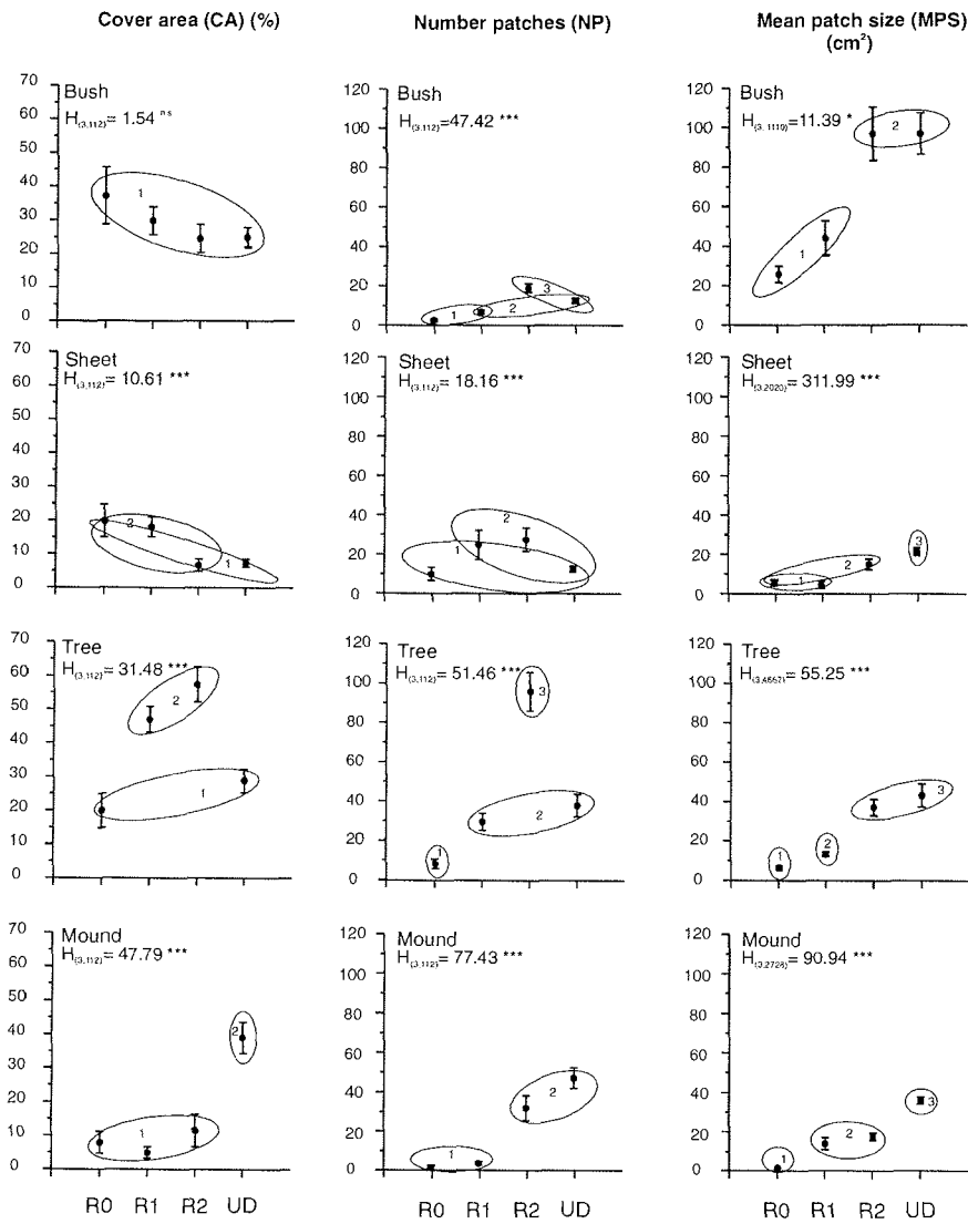
Fig. 4. Cover area (CA), number of patches (NP), and mean patch size (MPS) of growth form categories through succession. Homogeneous groups are enclosed with a circle according to Nemenyi post-hoc multiple comparisons. Data include mean \pm SE (standard error). See Table 2 for growth form descriptions. Note: The sum of different growth form categories exhibits ~ 85 % of cover area in R0 due to the absence of sessile benthic fauna in some photographs.
