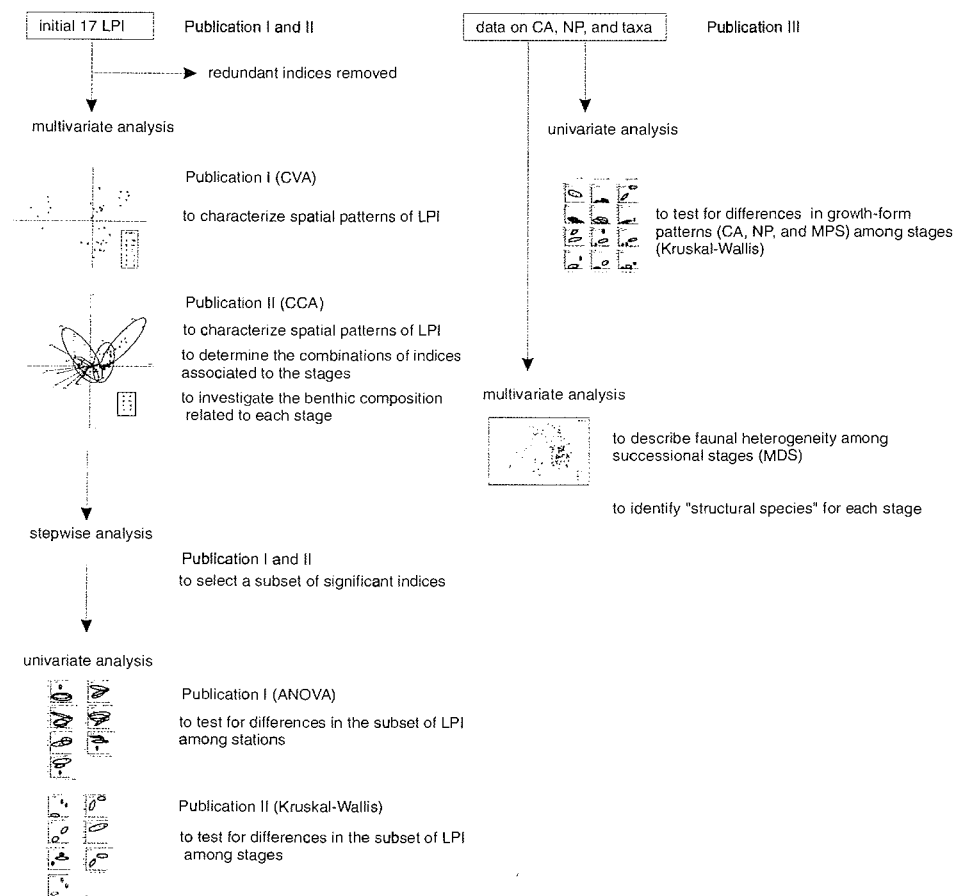
Fig. 7. General overview of the data analysis used in this study.
