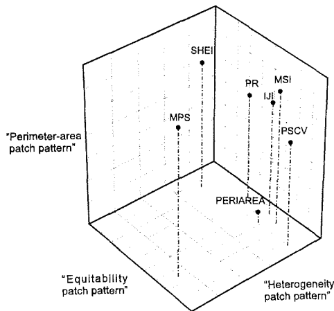
Fig. 4. 3D principal component analysis (PCA) of the subset of indices selected. The 3 first axes account for 84% of the variance. Mean patch size (MPS), patch size coefficient of variation (PSCV), mean shape index (MSI), periaerea index (PERIAREA), Shannon's evenness (SHEI), patch richness (PR), and interspersion and juxtaposition index (IJI)
